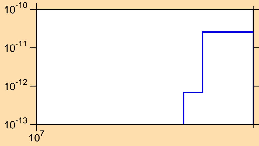
\sigma vs. E for ^{163}\text{Tm}(n,pd)
