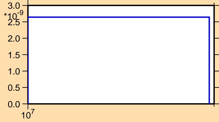
\sigma vs. E for ^{163}\text{Tm}(n,nt)
