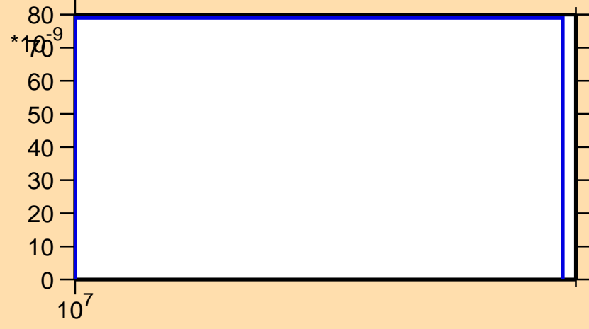
\sigma vs. E for ^{163}\text{Tm}(n,\text{nd})
