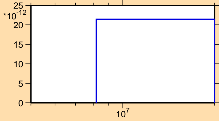
\sigma vs. E for ^{163}\text{Tm} (mt 45)
