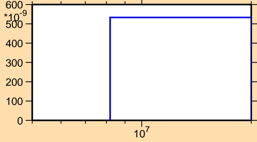
\sigma vs. E for ^{163}\text{Tm}(n,2np)
