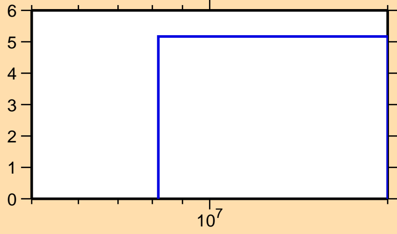
\Delta\sigma/\sigma vs. E for ^{163}\text{Tm}(n,\text{tot.})
