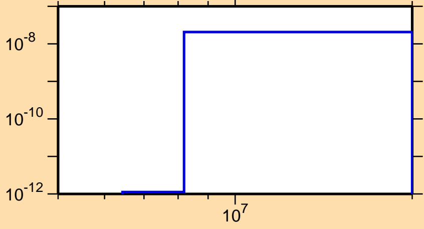
\sigma vs. E for ^{163}\text{Tm}(n,p\alpha)
