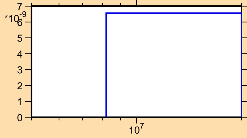
\sigma vs. E for ^{163}\text{Tm}(n,2n\alpha)
