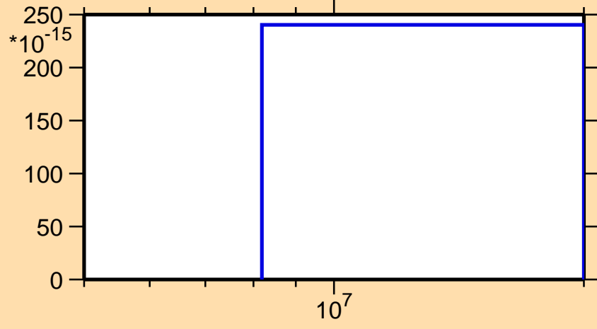
\sigma vs. E for ^{163}\text{Tm}(n,pd)
