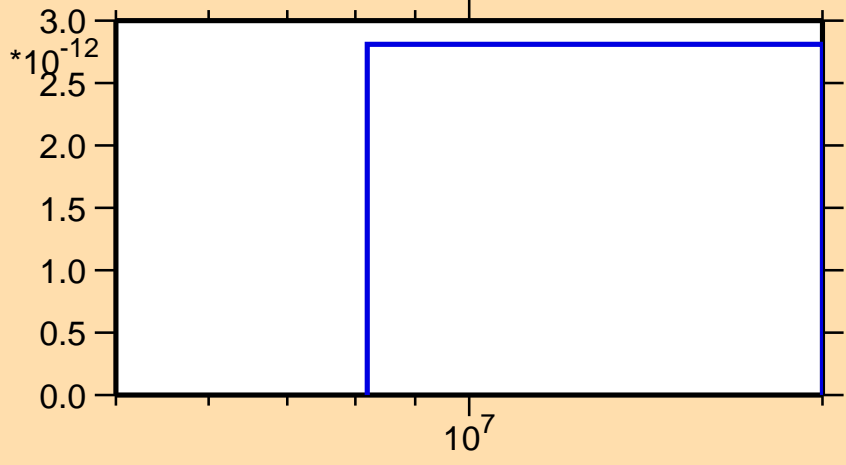
\sigma vs. E for ^{163}\text{Tm}(\text{mt117})
