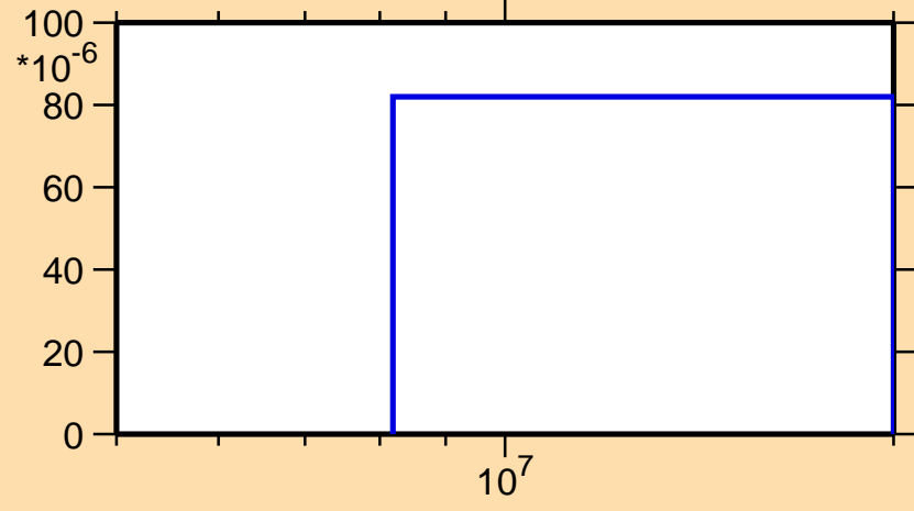
\sigma vs. E for ^{163}\text{Tm}(n,t)
