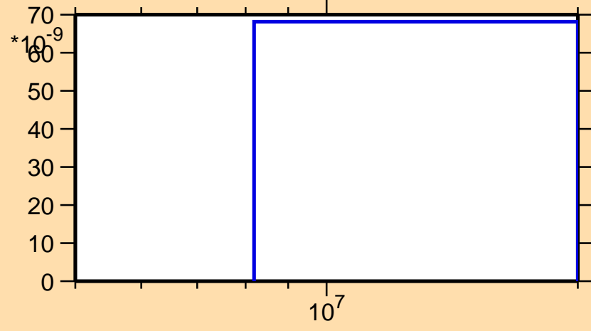
\sigma vs. E for ^{163}\text{Tm}(n,nd)
