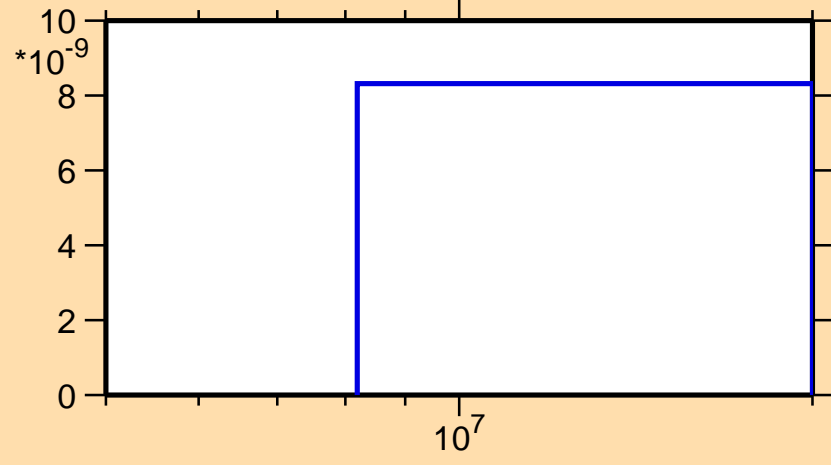
\sigma vs. E for ^{163}\text{Tm}(n,\text{He}3)
