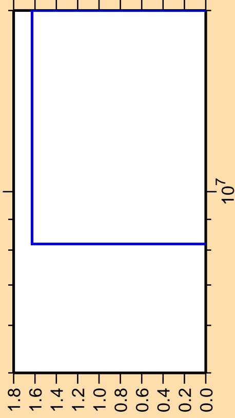
\Delta\sigma/\sigma vs. E for ^{163}\text{Tm}(n,pd)
