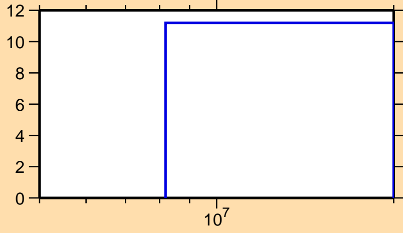
\Delta\sigma/\sigma vs. E for ^{163}\text{Tm}(n,\text{el.})
