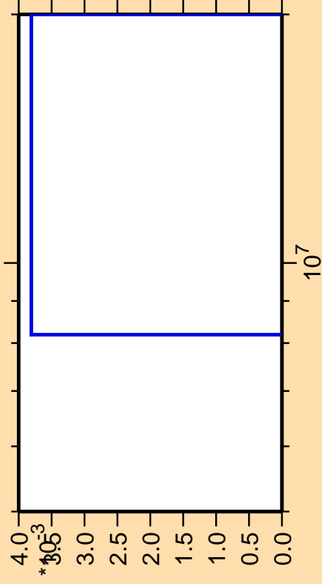
\Delta\sigma/\sigma vs. E for ^{163}\text{Tm} (mt 34)
