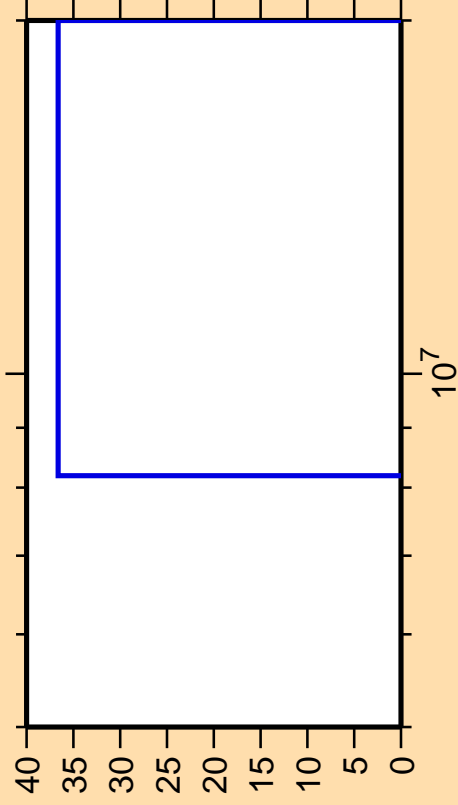
\Delta\sigma/\sigma vs. E for ^{163}\text{Tm}(n,2n)
