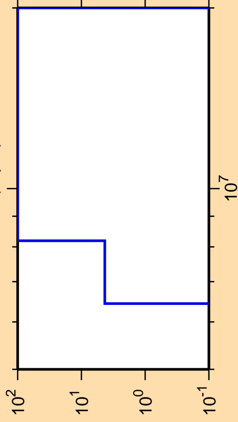
\Delta\sigma/\sigma vs. E for ^{163}\text{Tm}(n,p\alpha)
