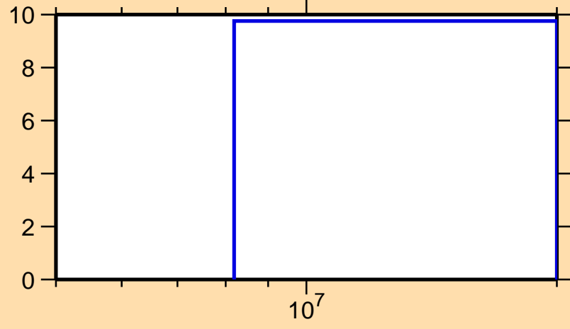
\Delta\sigma/\sigma vs. E for ^{163}\text{Tm}(n,\text{nonel.})
