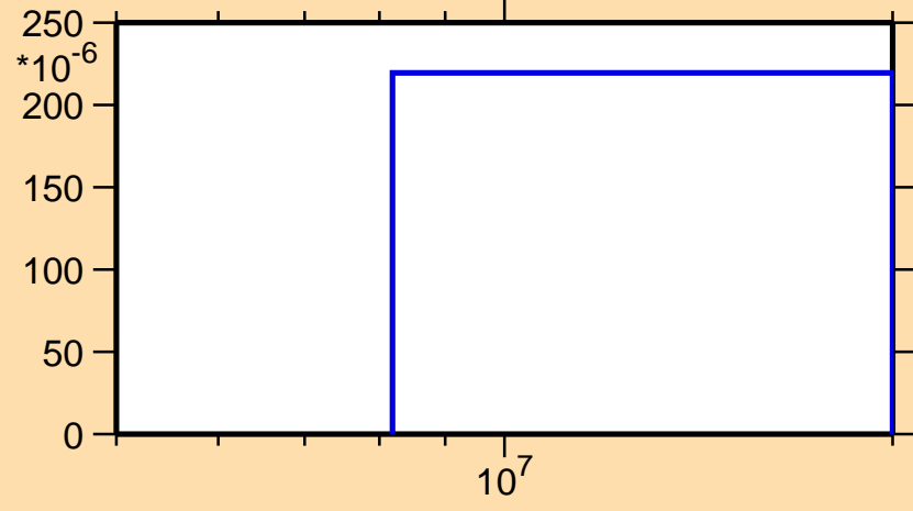
\sigma vs. E for ^{163}\text{Tm}(n,3n)
