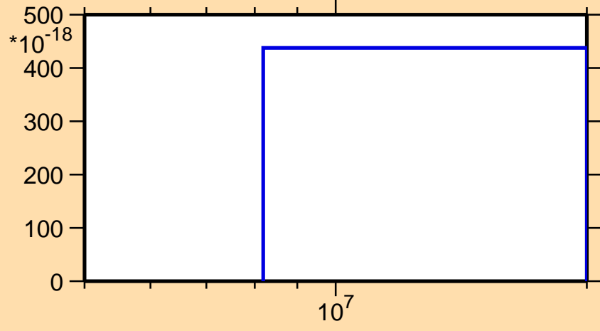
\sigma vs. E for ^{163}\text{Tm} (mt 34)
