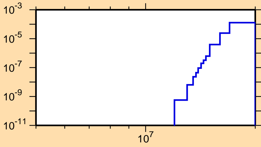
\sigma vs. E for ^{164}\text{Tm}(n,nd)
