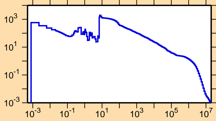
\sigma vs. E for ^{164}\text{Tm}(n,\gamma)
