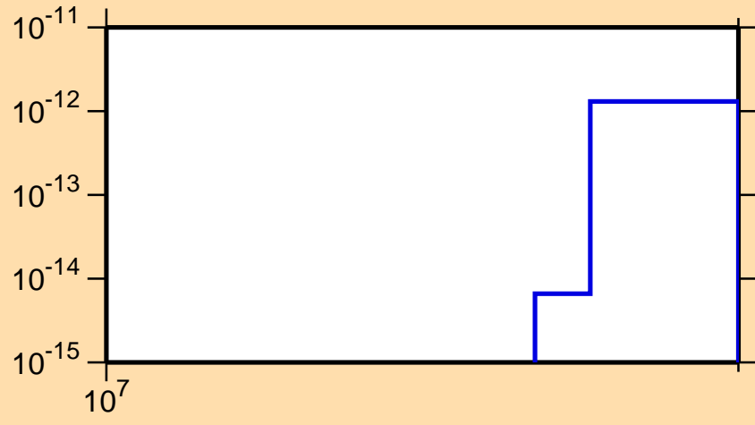
\sigma vs. E for ^{164}\text{Tm}(n,pt)
