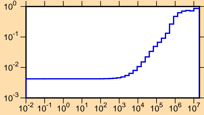
\mu vs. E for ^{164}\text{Tm}(\text{mt251})
