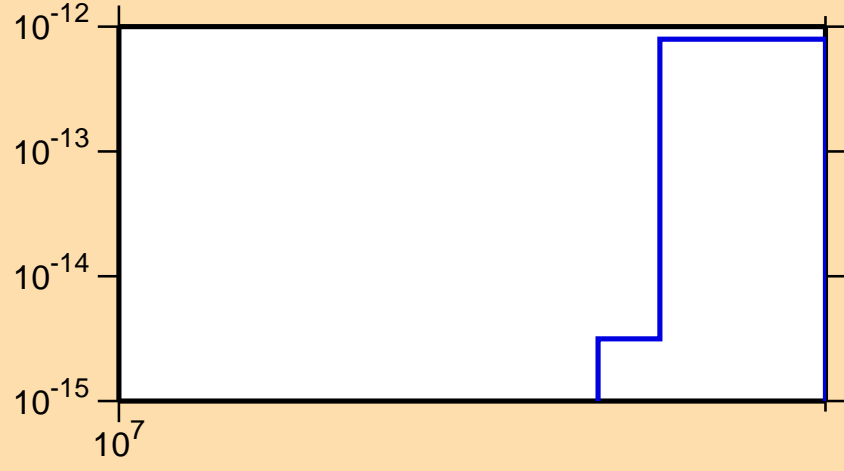
\sigma vs. E for ^{164}\text{Tm}(n,pt)
