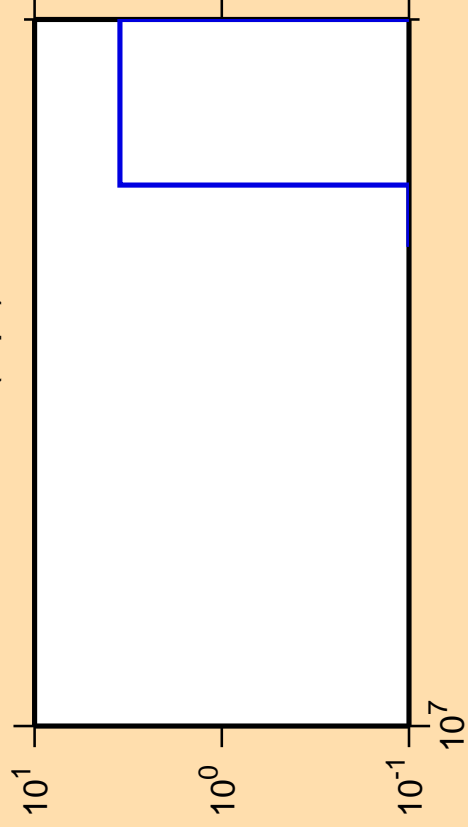
\Delta\sigma/\sigma vs. E for ^{164}\text{Tm}(n,pt)
