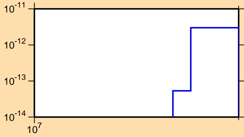
\sigma vs. E for ^{164}\text{Tm}(n,pd)
