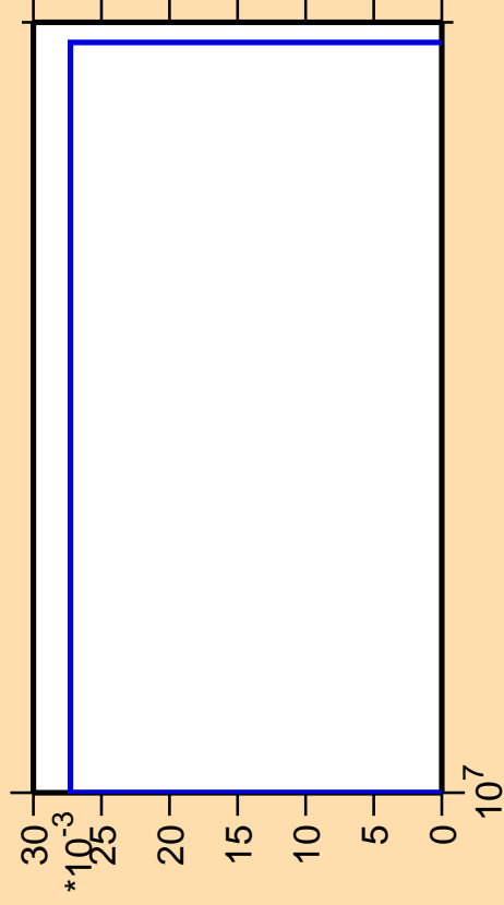
\Delta\sigma/\sigma vs. E for ^{164}\text{Tm}(n,pt)
