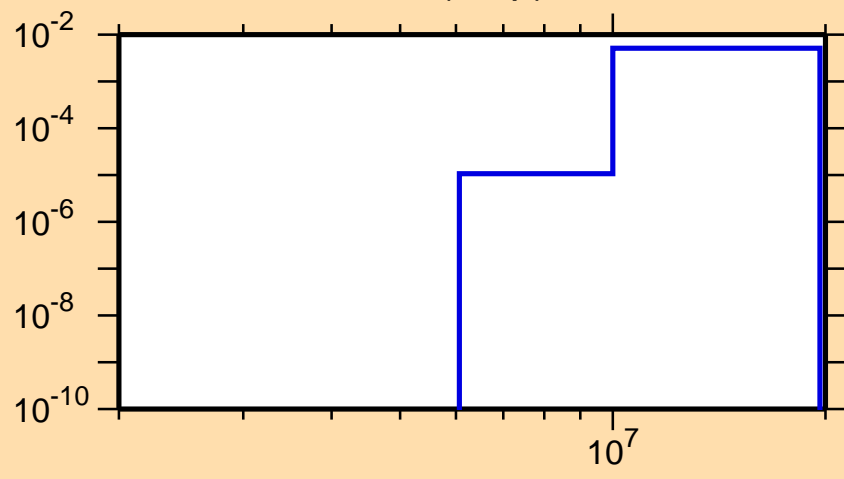
\sigma vs. E for ^{164}\text{Tm}(n,np)
