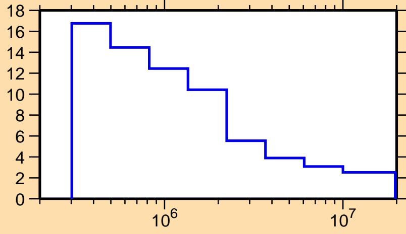
\Delta\sigma/\sigma vs. E for ^{164}\text{Tm}(n, n\text{onel.})
