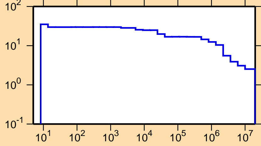
\Delta\sigma/\sigma vs. E for ^{164}\text{Tm}(n,\text{nonel.})
