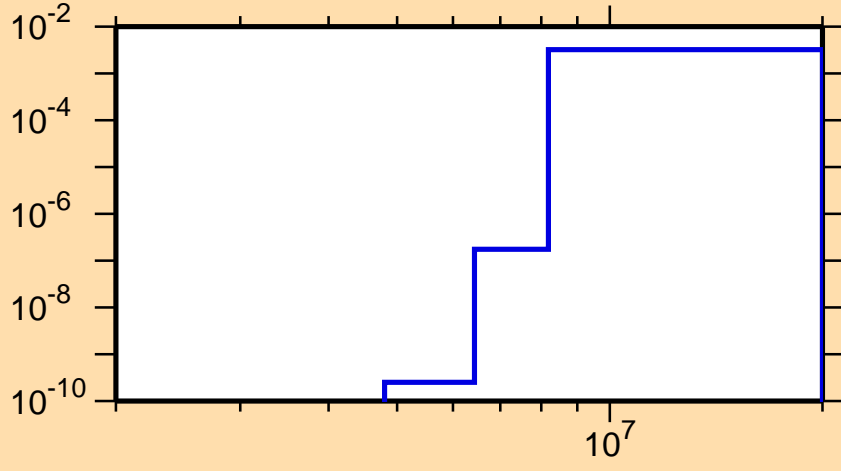
\sigma vs. E for ^{164}\text{Tm}(n,d)
