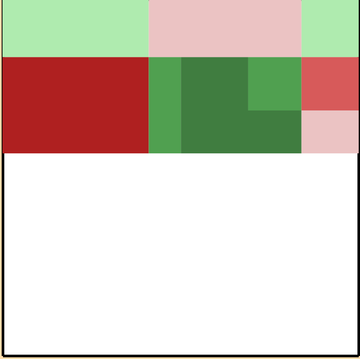
\Delta\sigma/\sigma vs. E for ^{165}\text{Tm}(n,\text{tot.})
