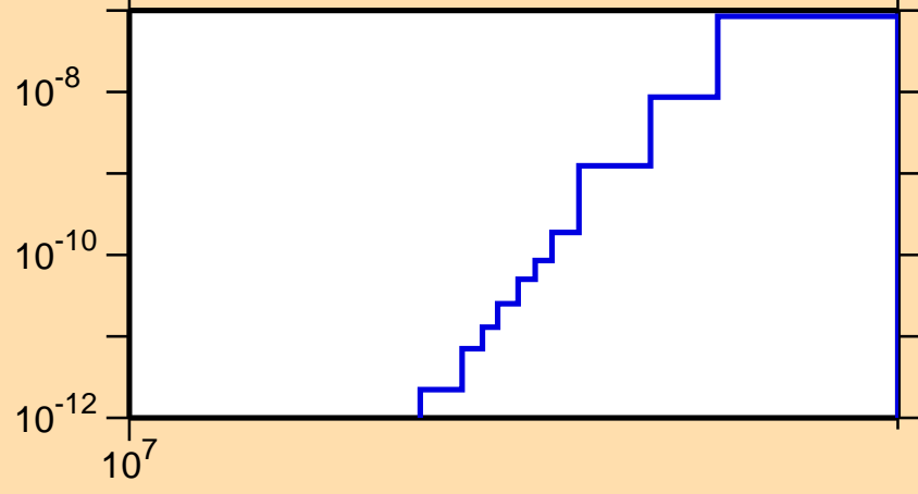
\sigma vs. E for ^{165}\text{Tm}(n,\text{He3})
