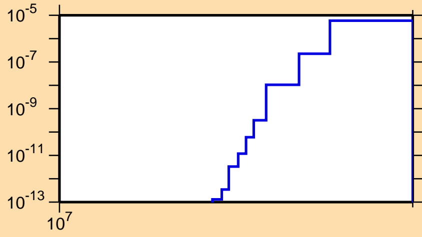
\sigma vs. E for ^{165}\text{Tm}(n,nd)
