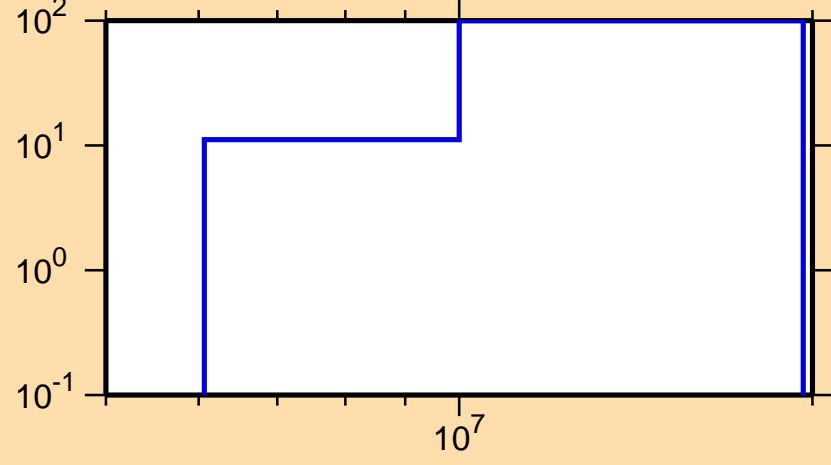
\Delta\sigma/\sigma vs. E for ^{165}\text{Tm}(n,\text{inel.})
