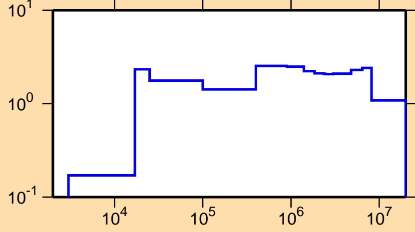
\sigma vs. E for ^{165}\text{Tm}(n,\text{inel.})
