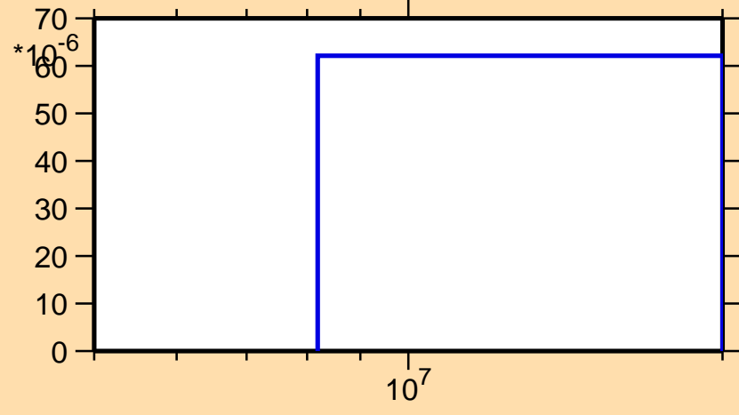
\sigma vs. E for ^{165}\text{Tm}(n,t)
