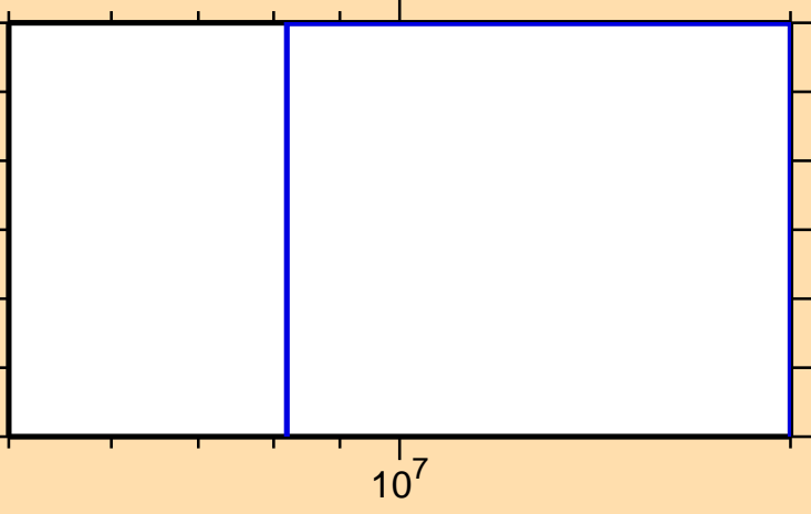
\sigma vs. E for ^{165}\text{Tm}(n,\text{He3})
