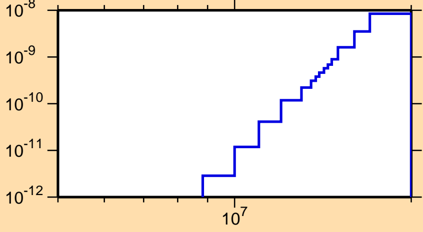
\sigma vs. E for ^{166}\text{Tm}(n,p\alpha)
