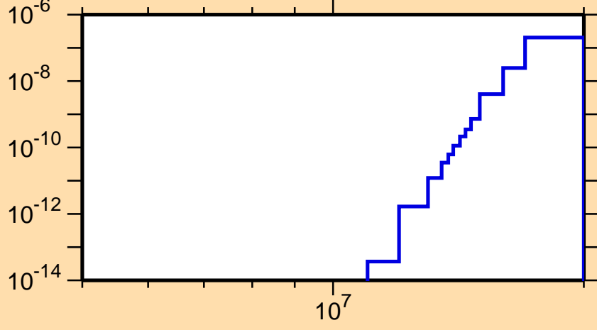
\sigma vs. E for ^{166}\text{Tm}(n,\text{He3})
