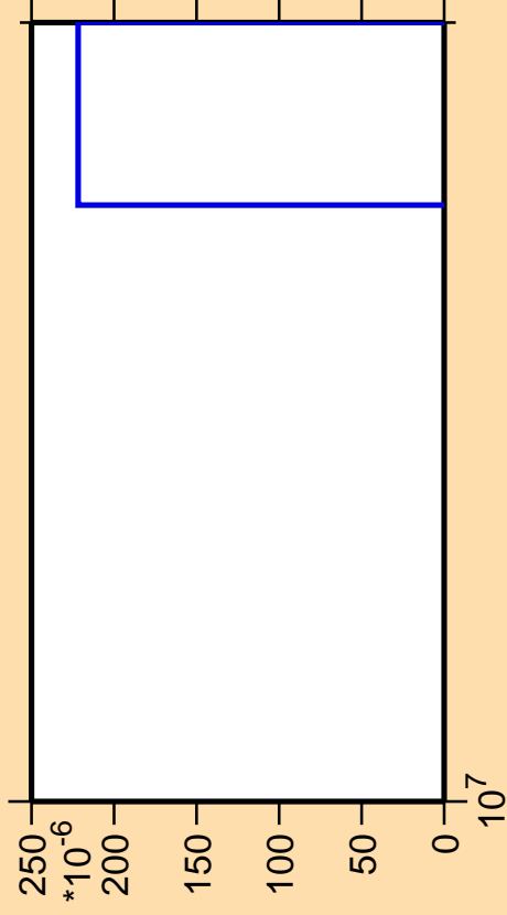
\Delta\sigma/\sigma vs. E for ^{166}\text{Tm} (mt 11)
