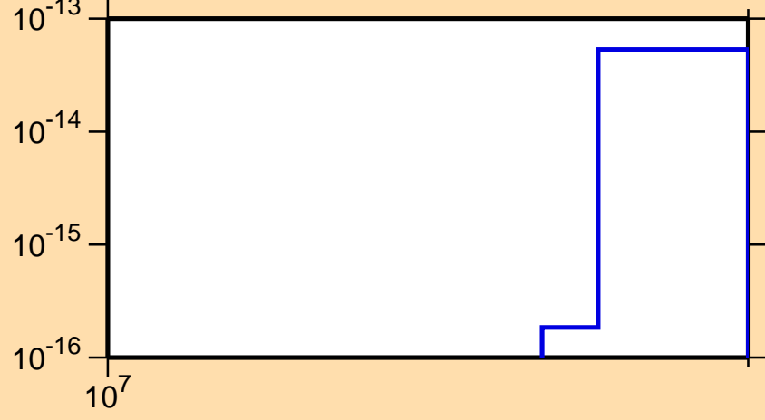
\sigma vs. E for ^{166}\text{Tm}(n,pd)
