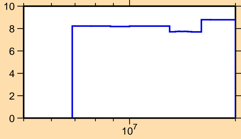
\Delta\sigma/\sigma vs. E for ^{166}\text{Tm}(n,\text{nonel.})
