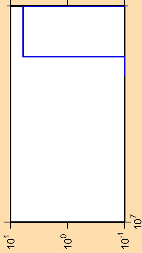
\Delta\sigma/\sigma vs. E for ^{166}\text{Tm} (mt 34)
