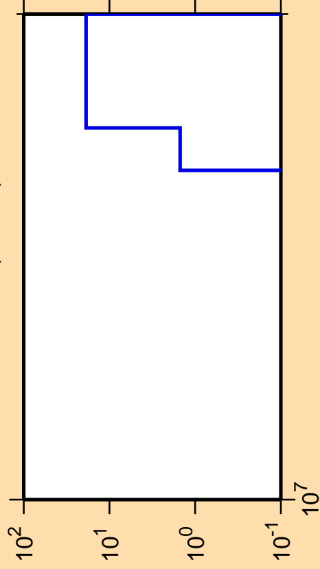
\Delta\sigma/\sigma vs. E for ^{166}\text{Tm} (mt 45)
