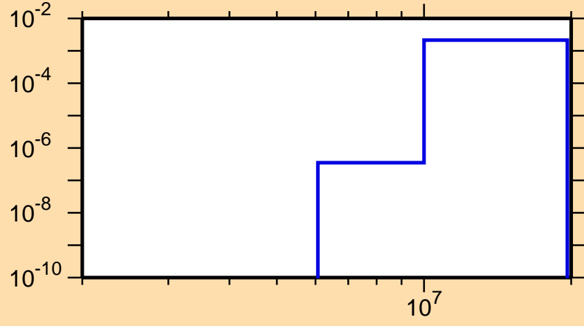
\sigma vs. E for ^{166}\text{Tm}(n,d)
