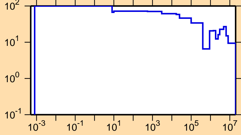
\Delta\sigma/\sigma vs. E for ^{166}\text{Tm}(n,\text{el.})
