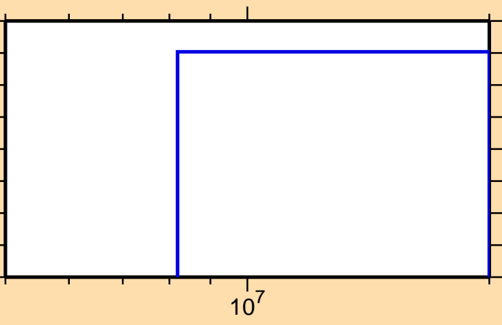
\sigma vs. E for ^{166}\text{Tm}(n,nd)
