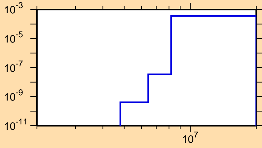
\sigma vs. E for ^{166}\text{Tm}(n,n\alpha)
