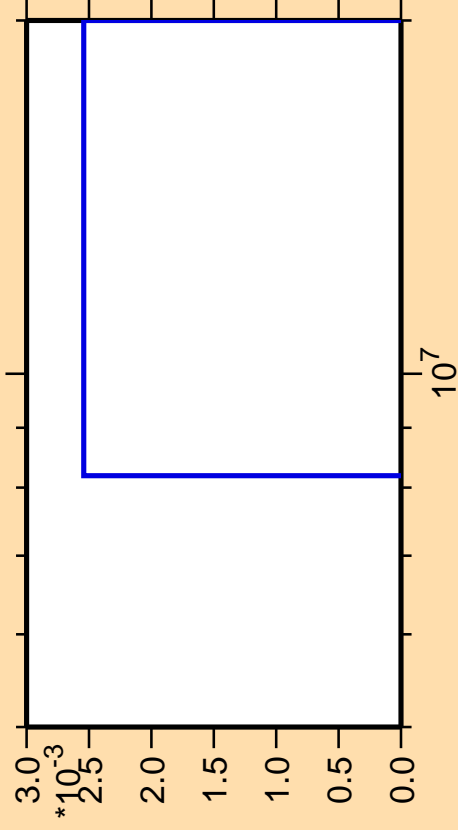
\Delta\sigma/\sigma vs. E for ^{166}\text{Tm}(n,pd)
