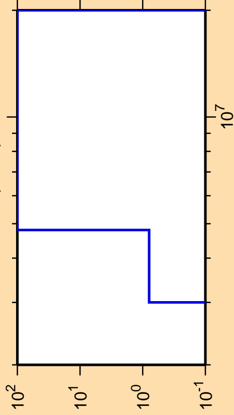
\Delta\sigma/\sigma vs. E for ^{166}\text{Tm}(n,n\alpha)
