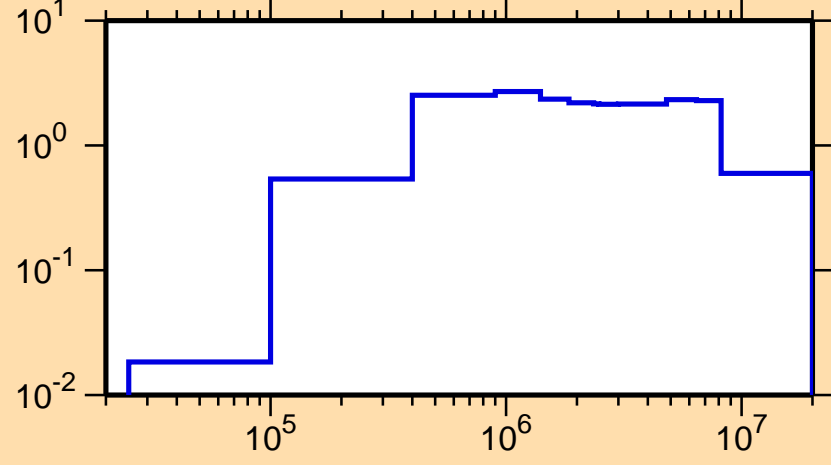
\sigma vs. E for ^{166}\text{Tm}(n,\text{inel.})
