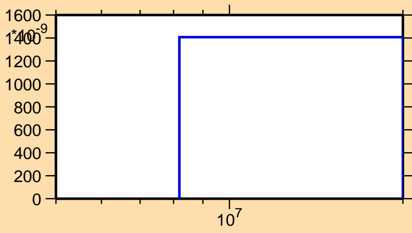
\sigma vs. E for ^{166}\text{Tm}(n,nd)
