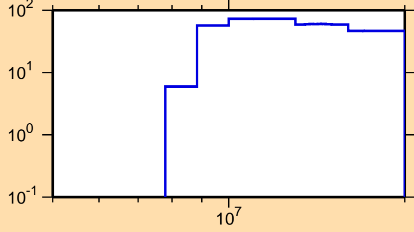
\Delta\sigma/\sigma vs. E for ^{167}\text{Tm}(n,\text{inel.})
