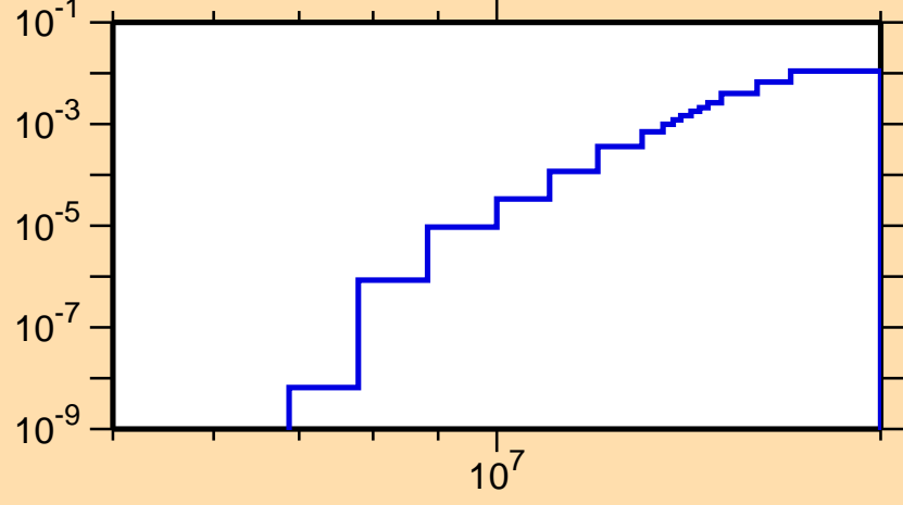
\sigma vs. E for ^{167}\text{Tm}(n,np)
