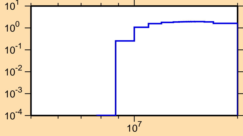
\sigma vs. E for ^{167}\text{Tm}(n,2n)
