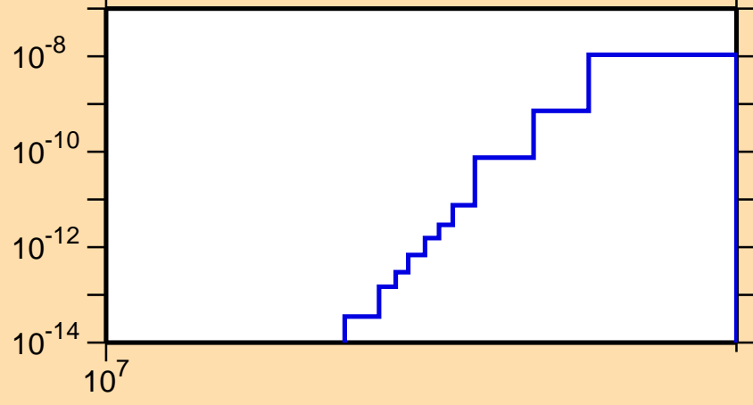
\sigma vs. E for ^{167}\text{Tm}(n,\text{He3})
