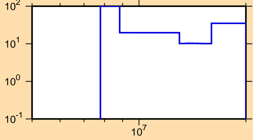
\Delta\sigma/\sigma vs. E for ^{167}\text{Tm}(n,2n)
