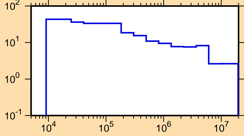
\Delta\sigma/\sigma vs. E for ^{167}\text{Tm}(n,\text{tot.})
