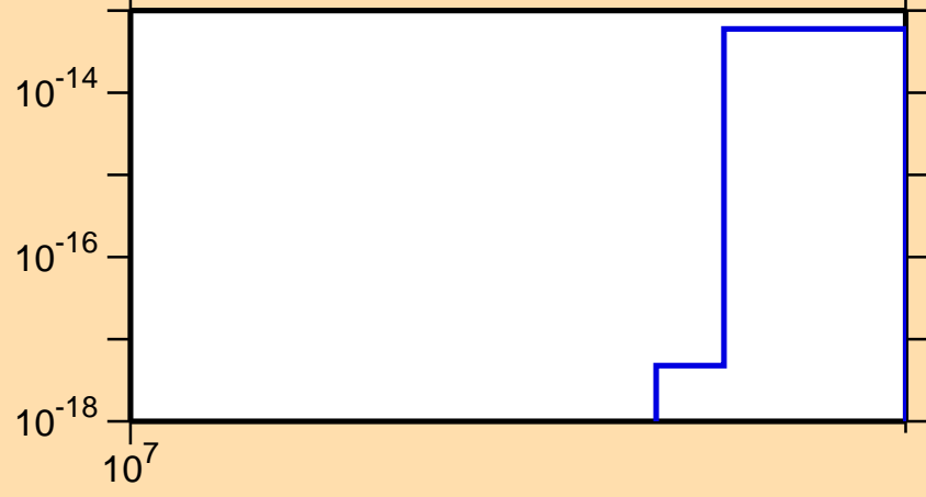
\sigma vs. E for ^{168}\text{Tm} (mt 34)
