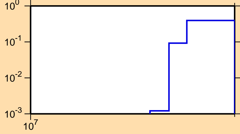
\sigma vs. E for ^{168}\text{Tm}(n,3n)
