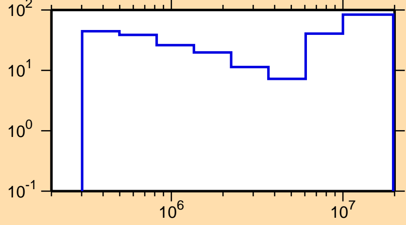
\Delta\sigma/\sigma vs. E for ^{168}\text{Tm}(n,\text{inel.})
