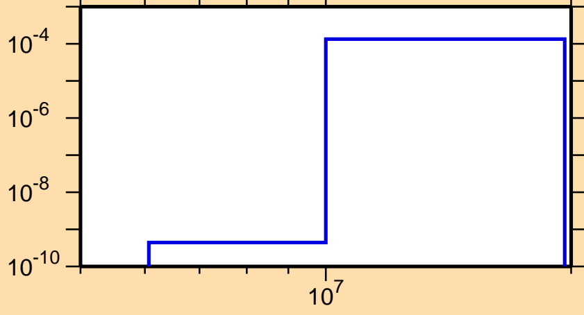
\sigma vs. E for ^{168}\text{Tm}(n,t)
