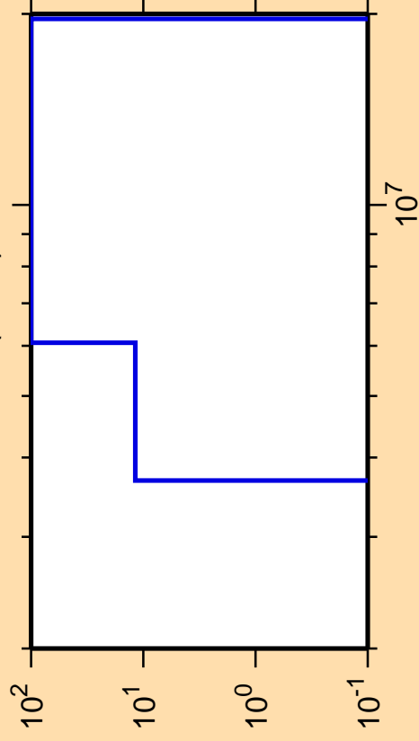
\Delta\sigma/\sigma vs. E for ^{168}\text{Tm}(n,n\alpha)
