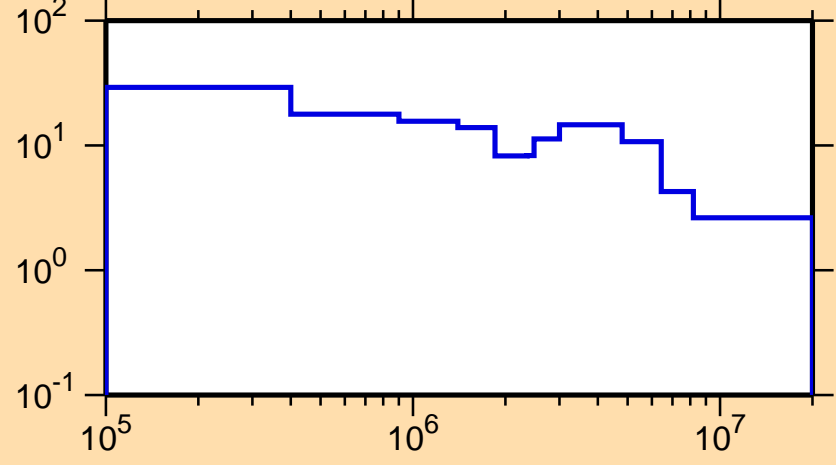
\Delta\sigma/\sigma vs. E for ^{168}\text{Tm}(n,\text{tot.})
