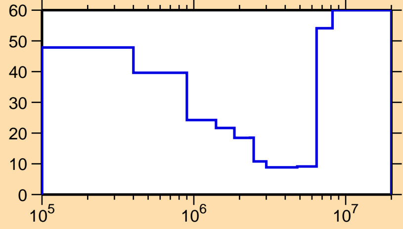
\Delta\sigma/\sigma vs. E for ^{168}\text{Tm}(n,inel.)
