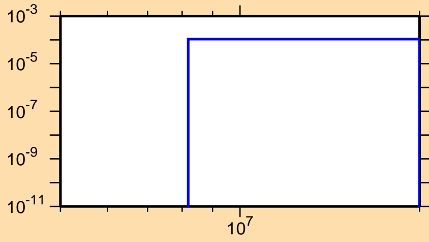
\sigma vs. E for ^{168}\text{Tm}(n,t)
