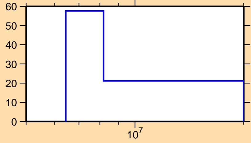
\Delta\sigma/\sigma vs. E for ^{168}\text{Tm}(n,2n)
