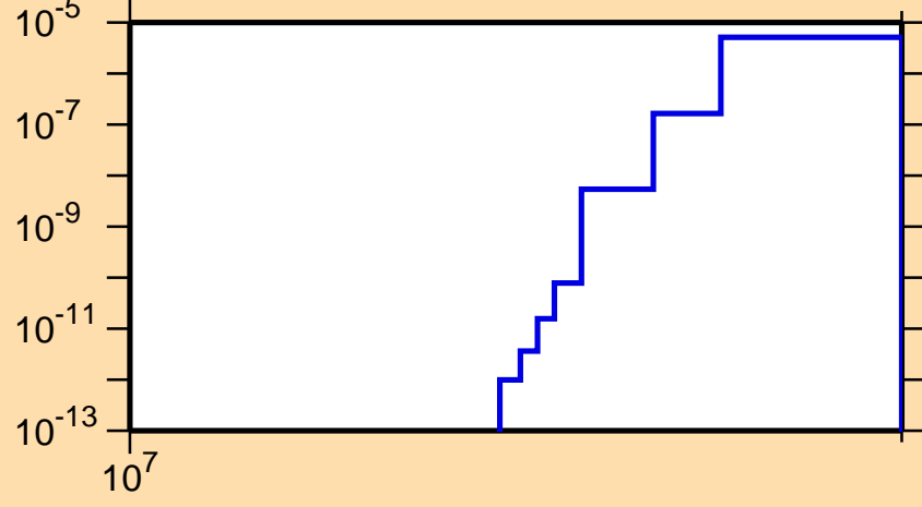
\sigma vs. E for ^{169}\text{Tm}(n,nd)
