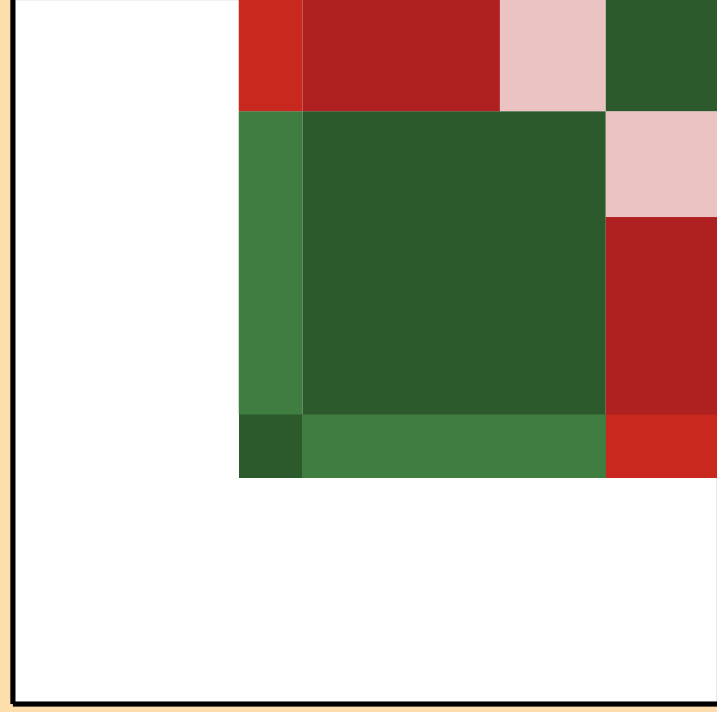
\sigma vs. E for ^{169}\text{Tm}(n,2n)
