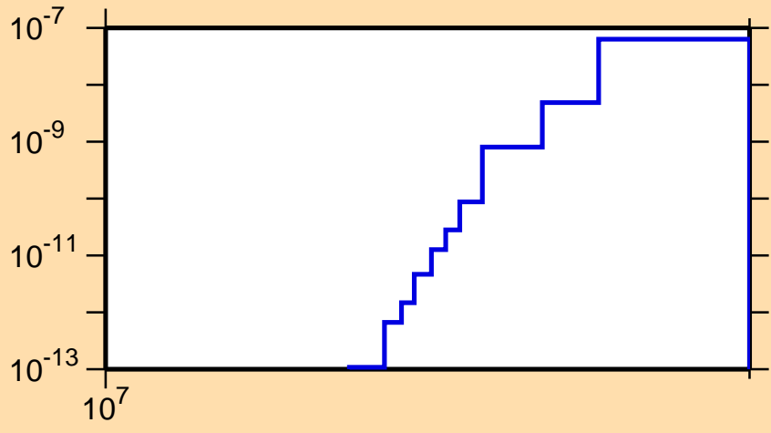
\sigma vs. E for ^{169}\text{Tm}(n,2n\alpha)
