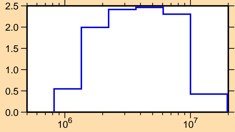
\sigma vs. E for ^{169}\text{Tm}(n,n\text{cont.})
