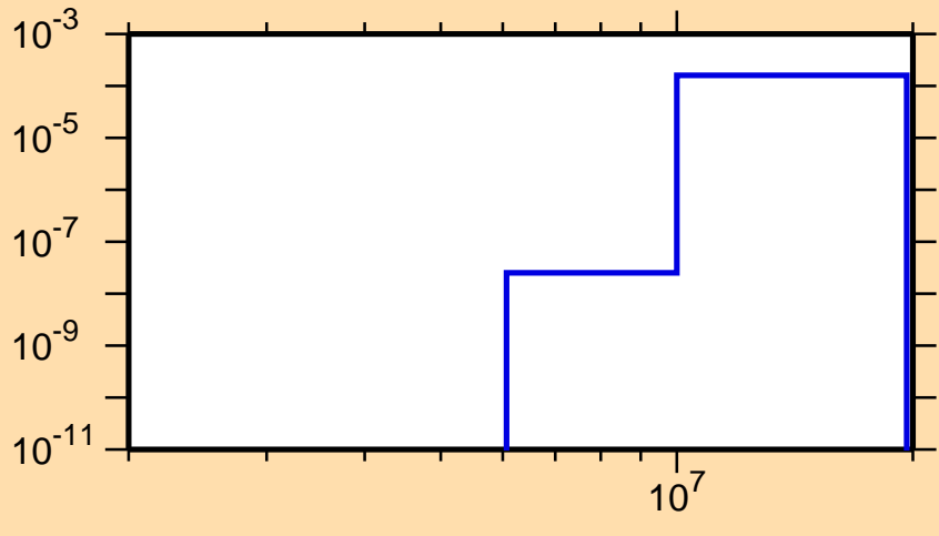
\sigma vs. E for ^{169}\text{Tm}(n,n\alpha)
