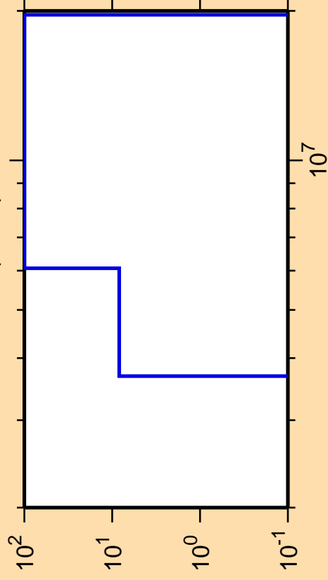
\Delta\sigma/\sigma vs. E for ^{169}\text{Tm}(n,n\alpha)
