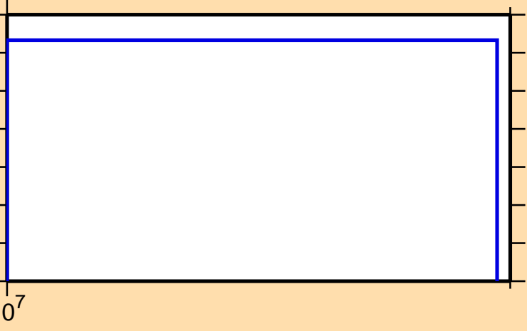
\sigma vs. E for ^{169}\text{Tm}(n,p\alpha)
