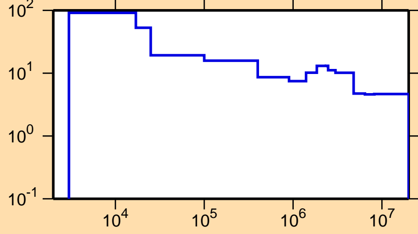
\Delta\sigma/\sigma vs. E for ^{169}\text{Tm}(n,\text{el.})
