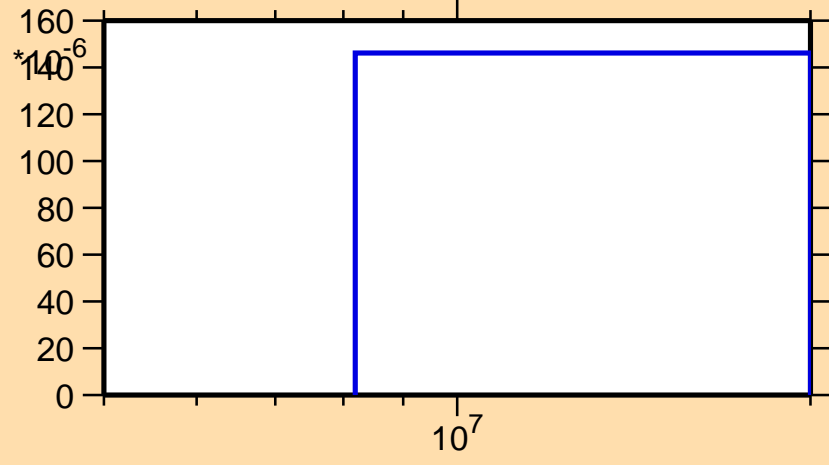
\sigma vs. E for ^{169}\text{Tm}(n,t)
