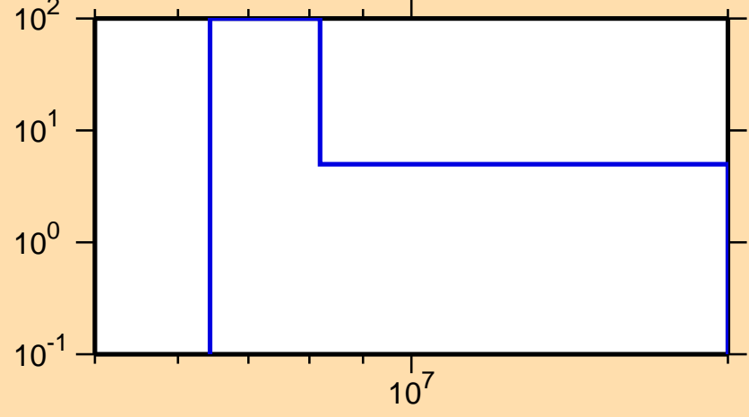
\Delta\sigma/\sigma vs. E for ^{169}\text{Tm}(n,2n)
