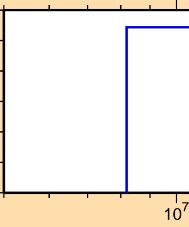
\sigma vs. E for ^{169}\text{Tm} (mt 42)
