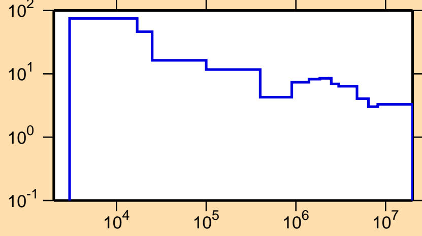
\Delta\sigma/\sigma vs. E for ^{169}\text{Tm}(n,\text{tot.})
