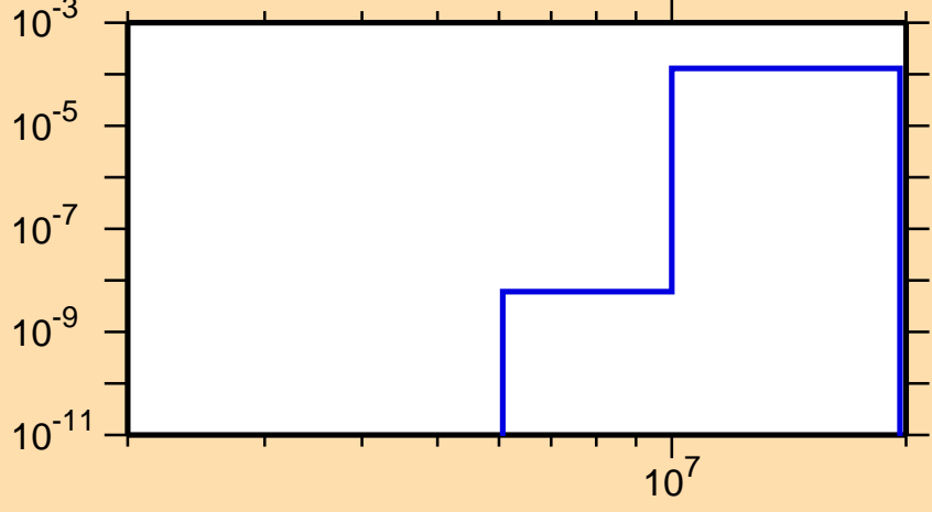
\sigma vs. E for ^{170}\text{Tm}(n,n\alpha)
