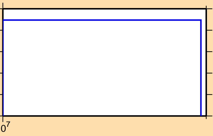
\sigma vs. E for ^{170}\text{Tm}(n,nd)
