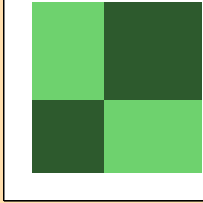
\sigma vs. E for ^{170}\text{Tm}(n,np)
