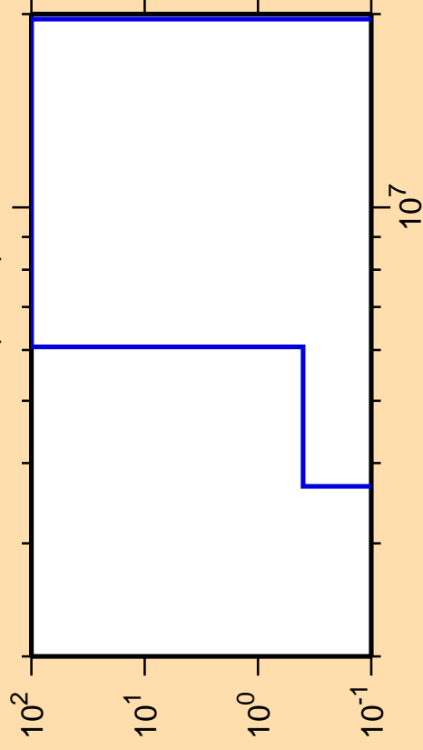
\Delta\sigma/\sigma vs. E for ^{170}\text{Tm}(n,n\alpha)
