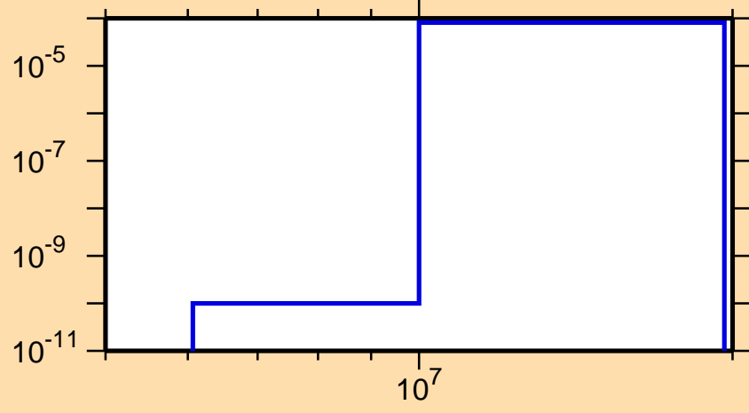
\sigma vs. E for ^{170}\text{Tm}(n,t)
