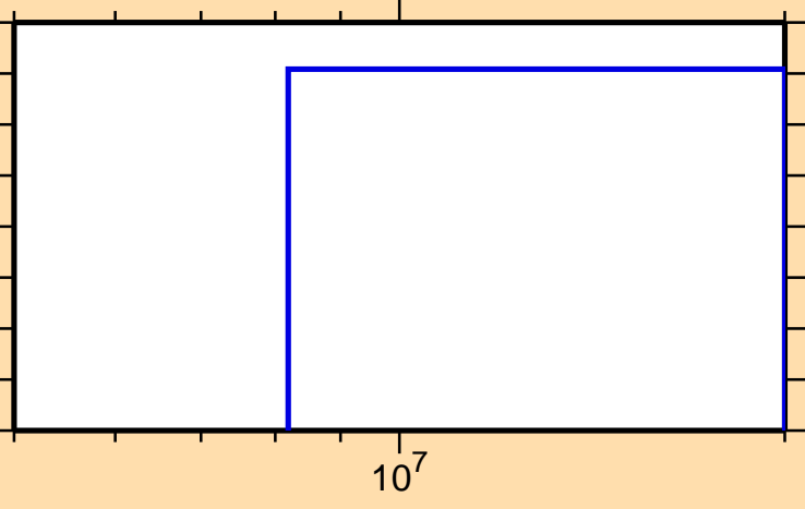
\sigma vs. E for ^{170}\text{Tm}(n,3n)
