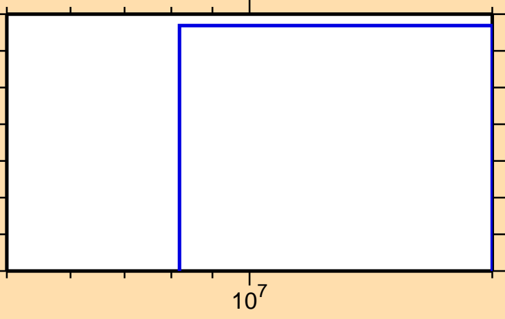
\sigma vs. E for ^{170}\text{Tm}(n,2n\alpha)
