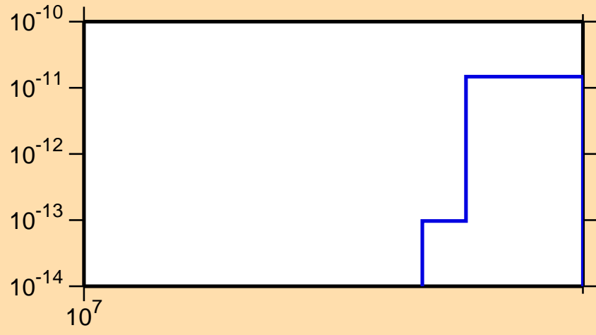
\sigma vs. E for ^{171}\text{Tm}(n,\text{He3})
