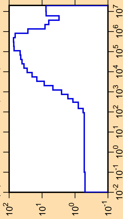
\Delta\mu/\mu vs. E for ^{171}\text{Tm}(\text{mt251})
