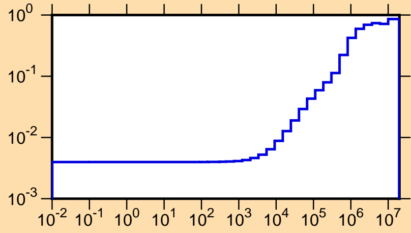
\mu vs. E for ^{171}\text{Tm}(\text{mt251})
