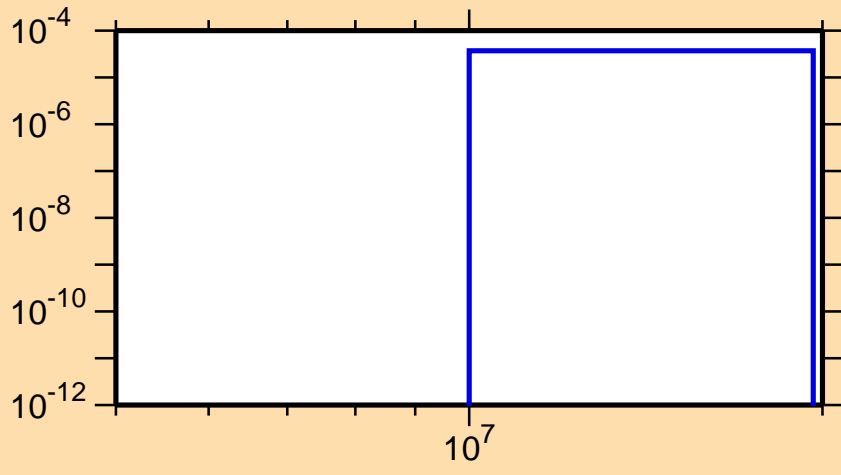
\sigma vs. E for ^{171}\text{Tm}(n,t)
