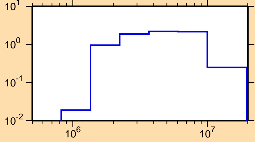
\sigma vs. E for ^{171}\text{Tm}(n,n\text{cont.})
