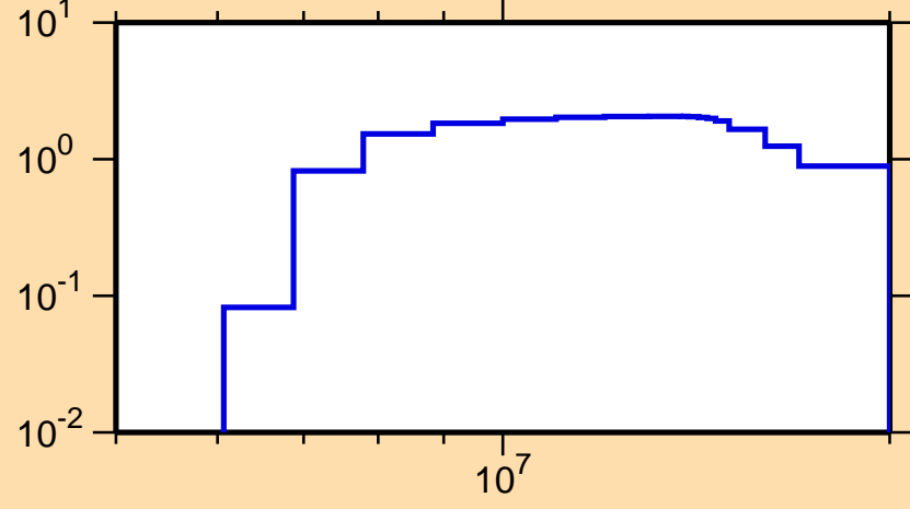
\sigma vs. E for ^{172}\text{Tm}(n,2n)
