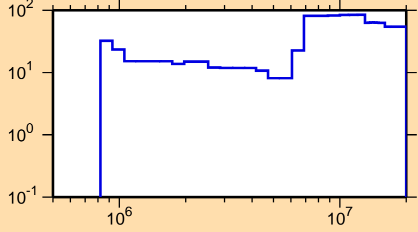
\Delta\sigma/\sigma vs. E for ^{172}\text{Tm}(n,\text{inel.})
