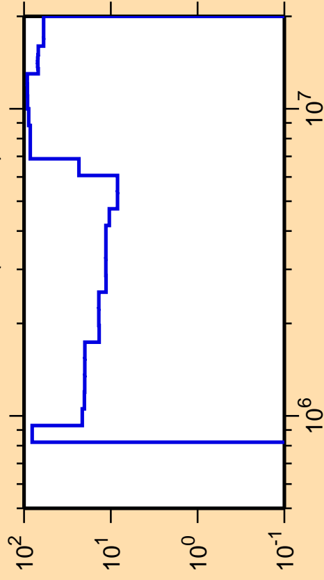
\Delta\sigma/\sigma vs. E for ^{172}\text{Tm}(n,n\text{cont.})
