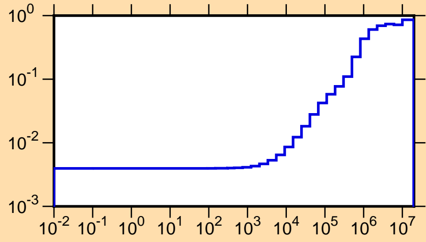
\mu vs. E for ^{172}\text{Tm}(\text{mt251})
