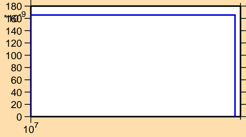
\sigma vs. E for ^{172}\text{Tm}(n,nd)
