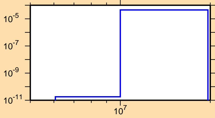
\sigma vs. E for ^{172}\text{Tm}(n,t)
