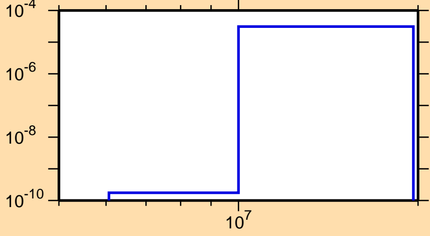
\sigma vs. E for ^{172}\text{Tm}(n,\alpha)
