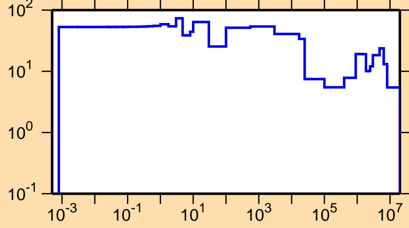
\Delta\sigma/\sigma vs. E for ^{172}\text{Tm}(n,\text{el.})
