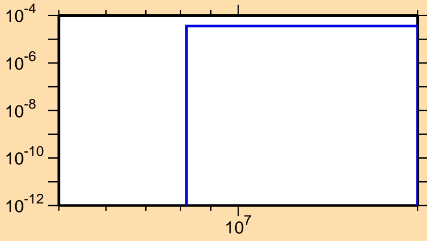
\sigma vs. E for ^{172}\text{Tm}(n,t)
