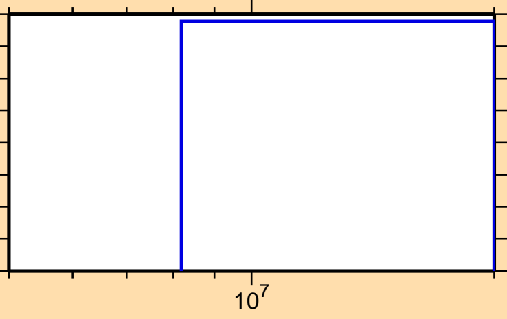
\sigma vs. E for ^{172}\text{Tm} (mt 42)
