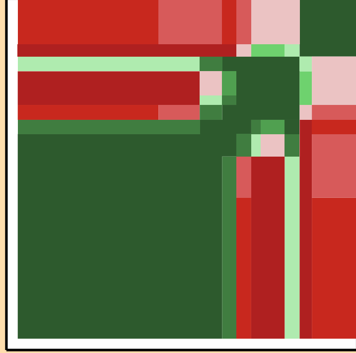
\sigma vs. E for ^{172}\text{Tm}(n,\text{inel.})
