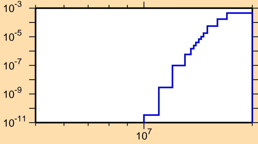
\sigma vs. E for ^{173}\text{Tm}(n,t)
