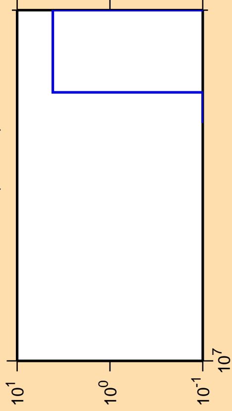
\Delta\sigma/\sigma vs. E for ^{173}\text{Tm}(n,\text{He3})
