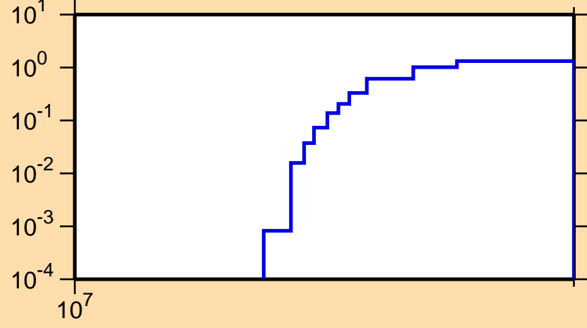
\sigma vs. E for ^{173}\text{Tm}(n,3n)
