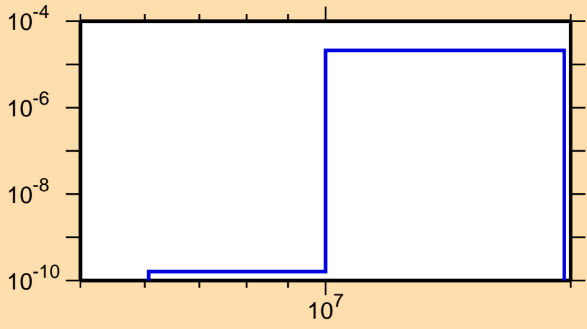
\sigma vs. E for ^{173}\text{Tm}(n,\alpha)
