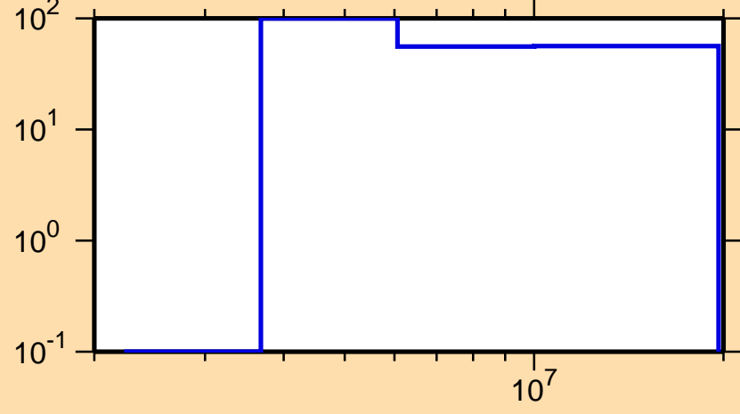
\Delta\sigma/\sigma vs. E for ^{173}\text{Tm}(n,p)
