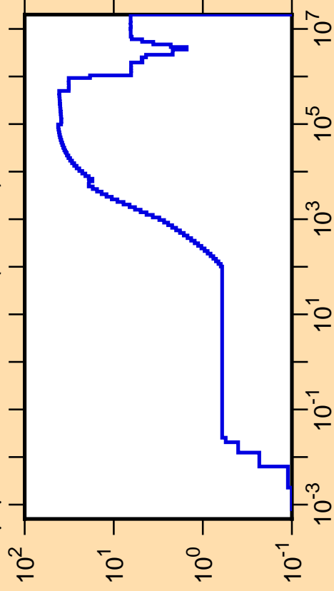
\Delta\mu/\mu vs. E for ^{174}\text{Tm}(\text{mt251})
