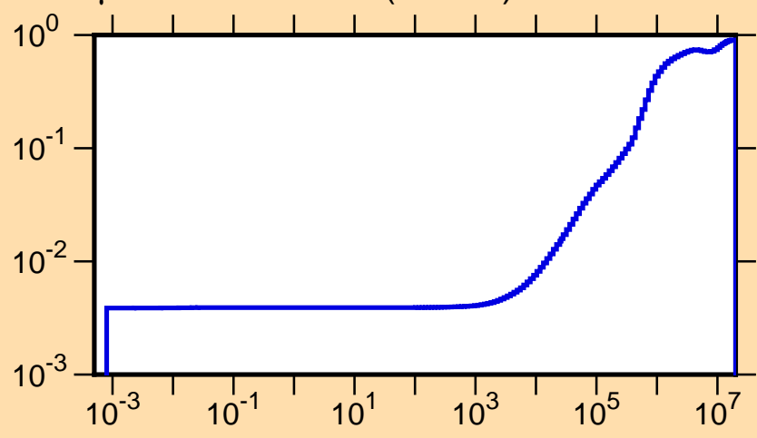
\mu vs. E for ^{174}\text{Tm}(\text{mt251})
