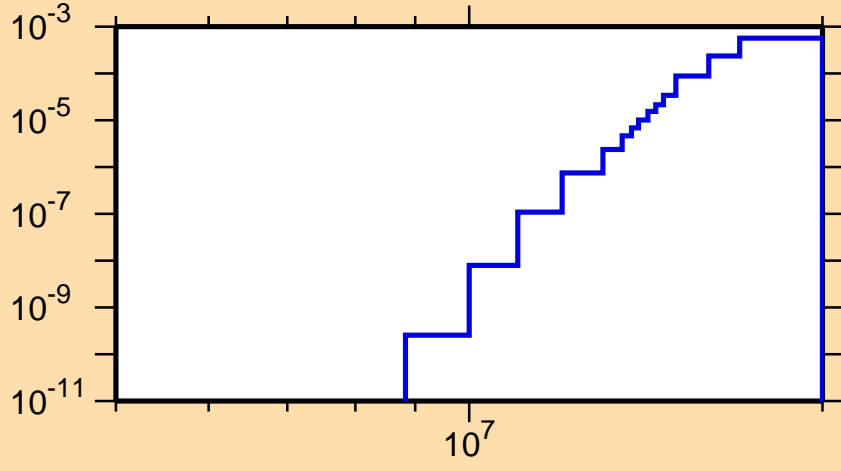
\sigma vs. E for ^{174}\text{Tm}(n,t)
