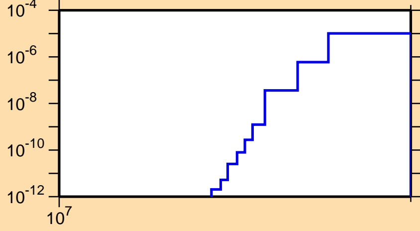
\sigma vs. E for ^{174}\text{Tm}(n,nd)
