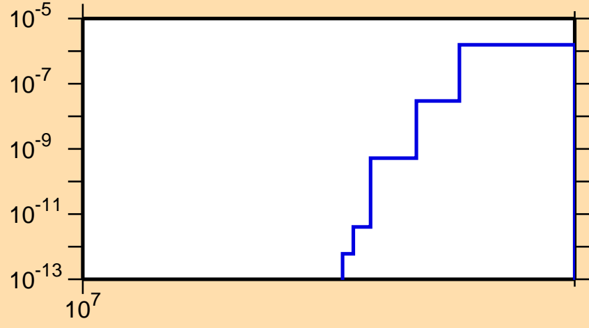
\sigma vs. E for ^{174}\text{Tm}(n,2np)
