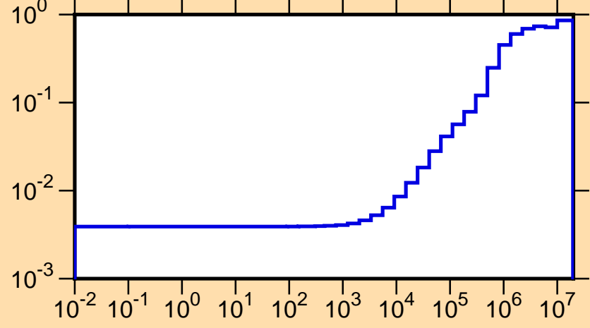
\mu vs. E for ^{174}\text{Tm}(\text{mt251})
