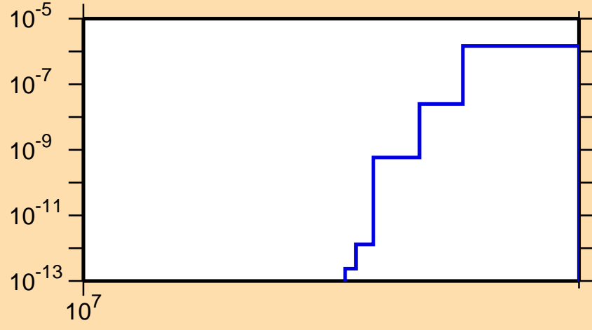
\sigma vs. E for ^{175}\text{Tm}(n,nd)
