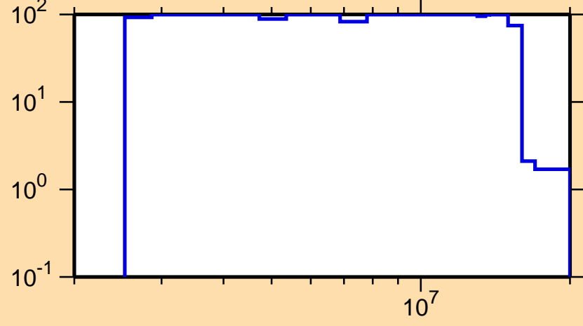
\Delta\sigma/\sigma vs. E for ^{175}\text{Tm}(n,n_1)
