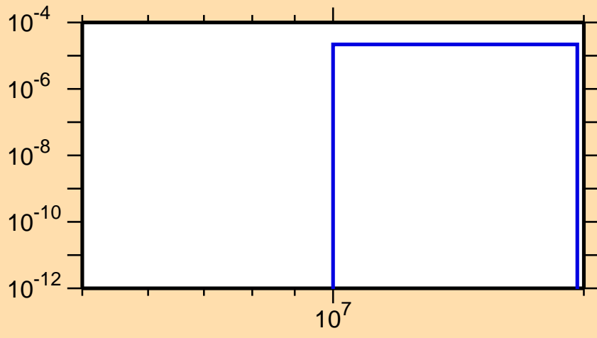
\sigma vs. E for ^{175}\text{Tm}(n,t)
