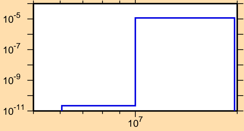
\sigma vs. E for ^{175}\text{Tm}(n,\alpha)
