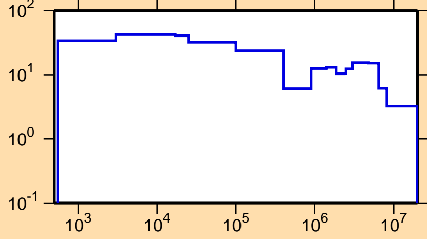
\Delta\sigma/\sigma vs. E for ^{175}\text{Tm}(n,\text{el.})
