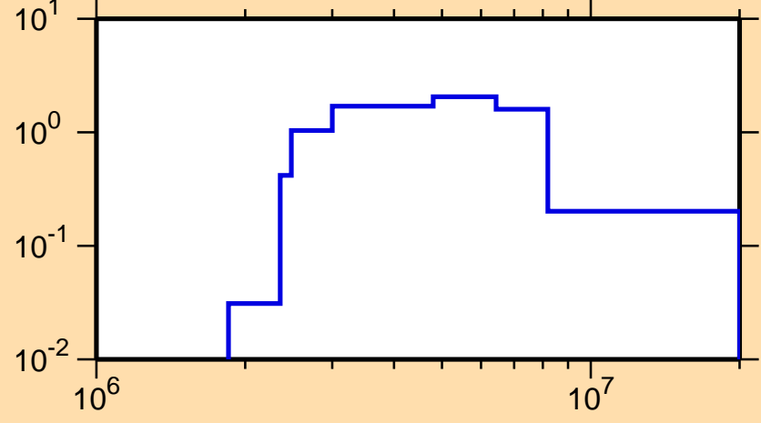
\sigma vs. E for ^{175}\text{Tm}(n,n\text{cont.})
