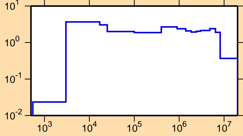
\sigma vs. E for ^{175}\text{Tm}(n,\text{inel.})
