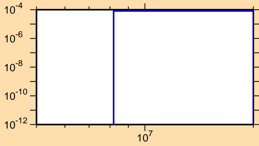
\sigma vs. E for ^{175}\text{Tm}(n,np)
