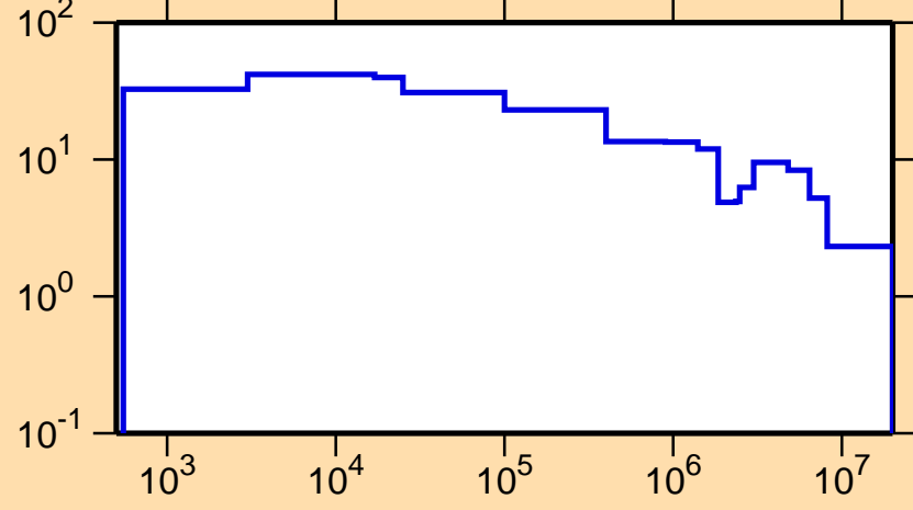
\Delta\sigma/\sigma vs. E for ^{175}\text{Tm}(n,\text{tot.})
