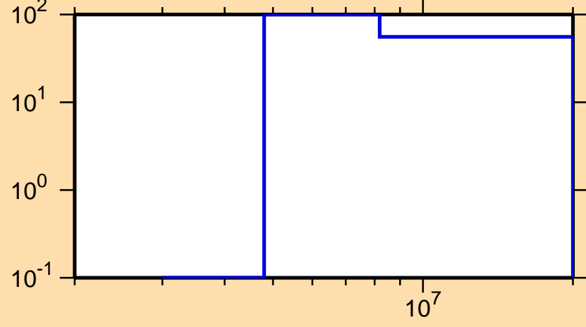
\Delta\sigma/\sigma vs. E for ^{175}\text{Tm}(n,p)
