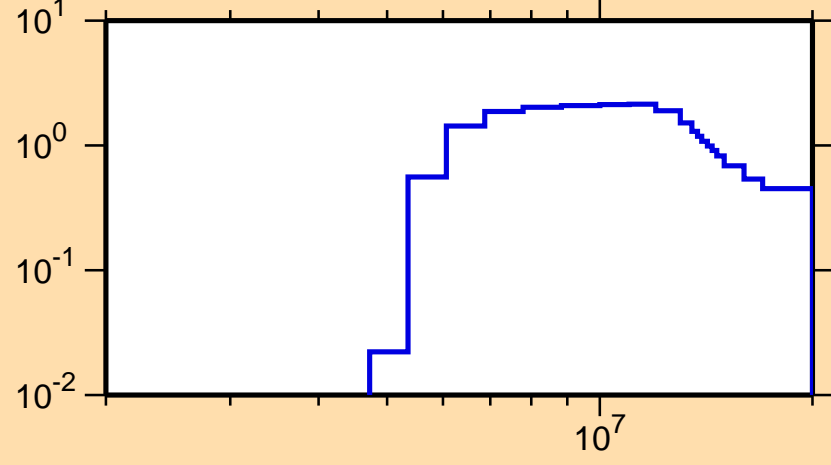
\sigma vs. E for ^{176}\text{Tm}(n,2n)
