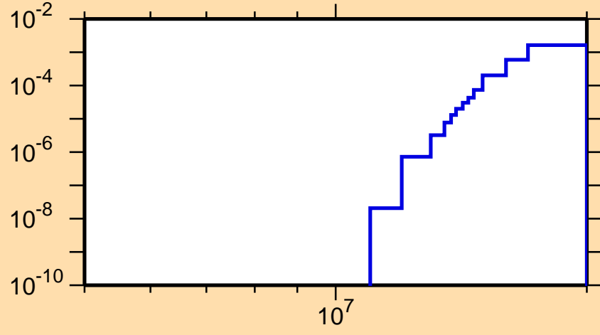
\sigma vs. E for ^{176}\text{Tm}(n,np)
