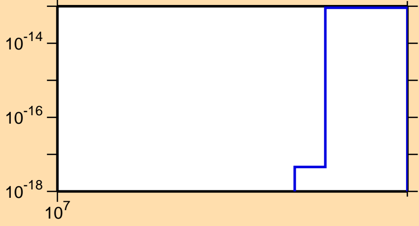
\sigma vs. E for ^{176}\text{Tm}(n,3n\alpha)
