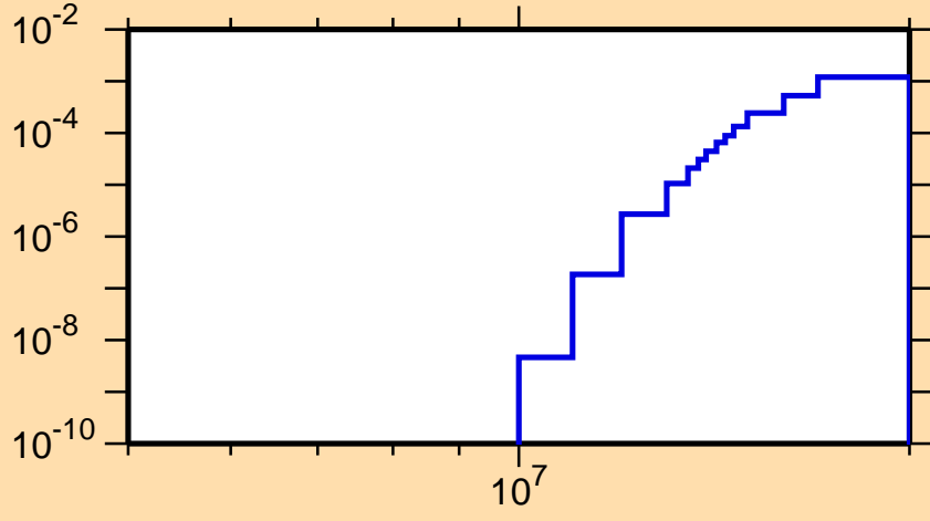
\sigma vs. E for ^{176}\text{Tm}(n,d)
