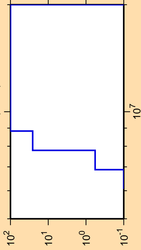
\Delta\sigma/\sigma vs. E for ^{176}\text{Tm}(n,n\alpha)
