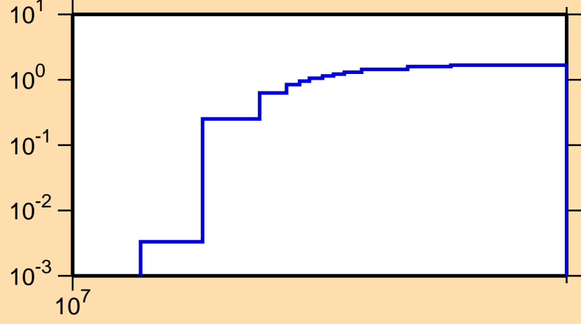
\sigma vs. E for ^{176}\text{Tm}(n,3n)
