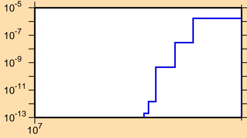
\sigma vs. E for ^{176}\text{Tm}(n,2np)
