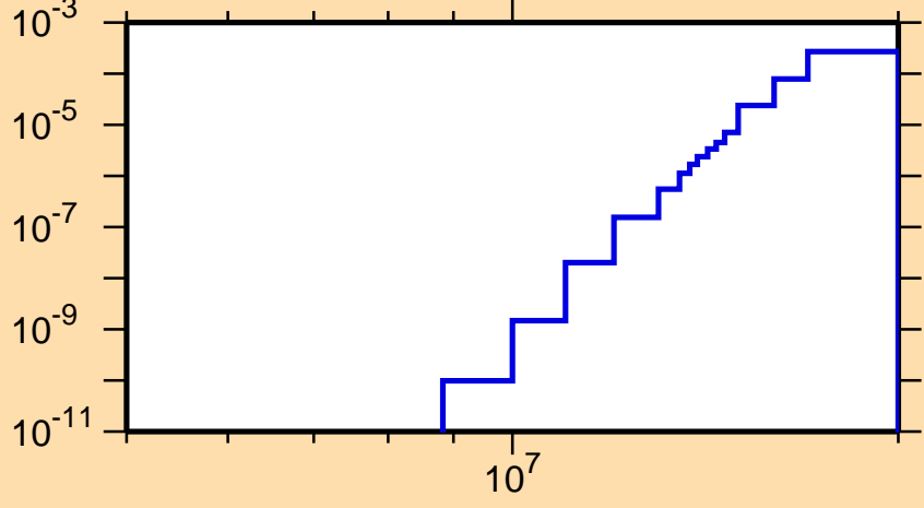
\sigma vs. E for ^{176}\text{Tm}(n,n\alpha)
