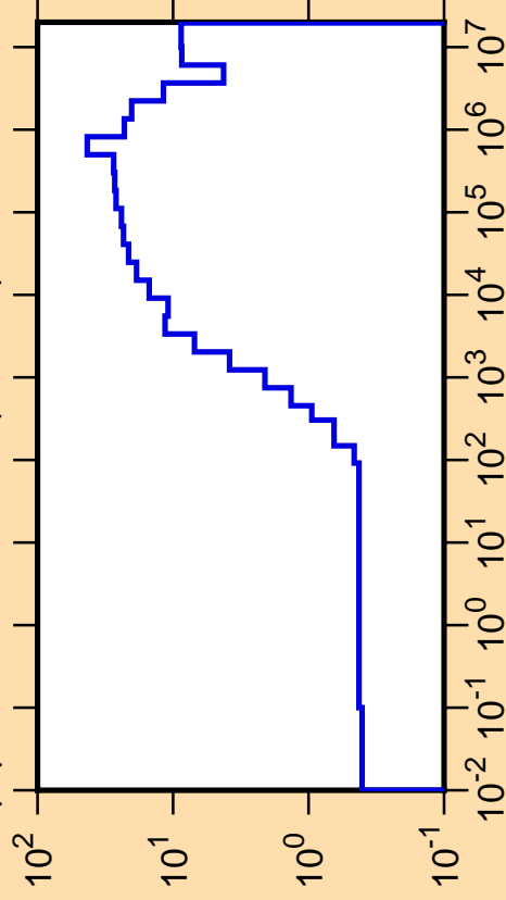
\Delta\mu/\mu vs. E for ^{176}\text{Tm}(\text{mt251})
