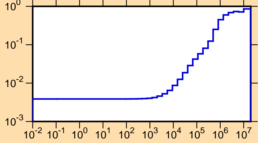
\mu vs. E for ^{176}\text{Tm}(\text{mt251})
