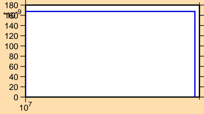
\sigma vs. E for ^{176}\text{Tm}(n,nd)
