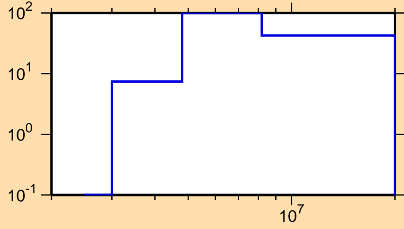
\Delta\sigma/\sigma vs. E for ^{176}\text{Tm}(n,p)
