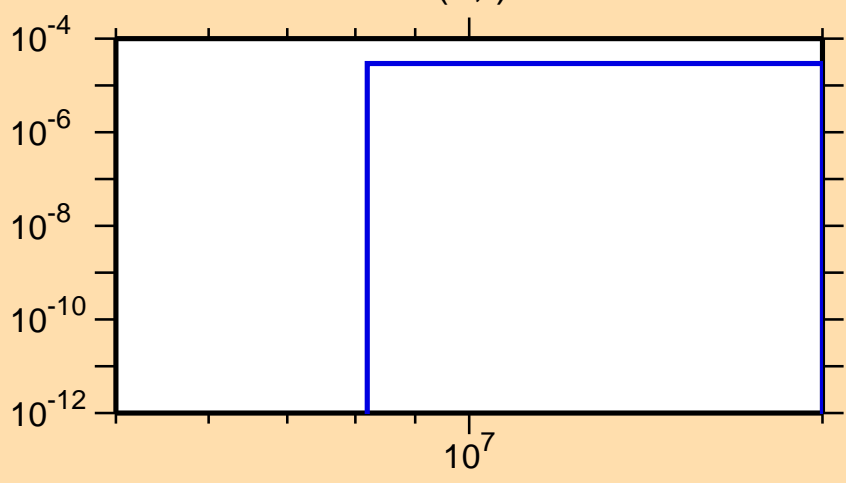
\sigma vs. E for ^{176}\text{Tm}(n,t)
