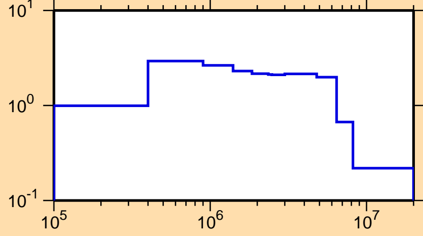
\sigma vs. E for ^{176}\text{Tm}(n,\text{inel.})
