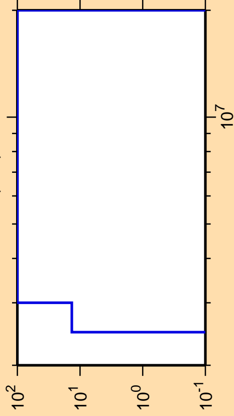
\Delta\sigma/\sigma vs. E for ^{176}\text{Tm}(n,\alpha)
