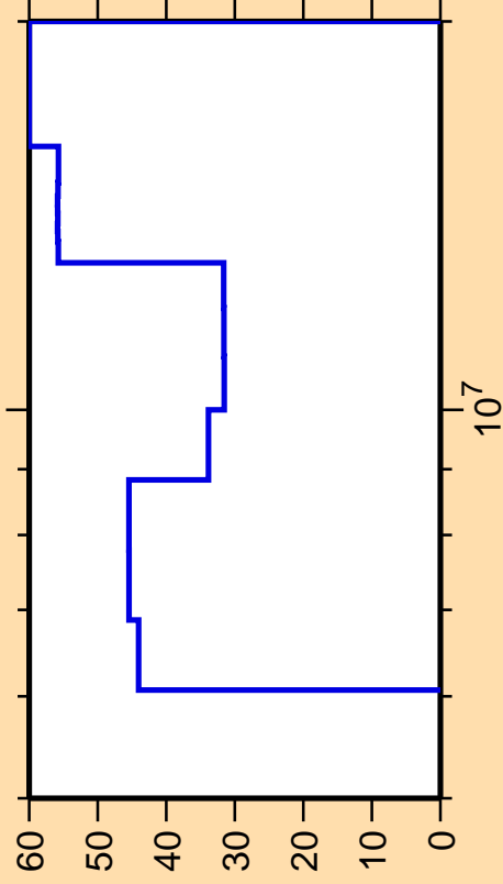
\Delta\sigma/\sigma vs. E for ^{177}\text{Tm}(n,n_1)
