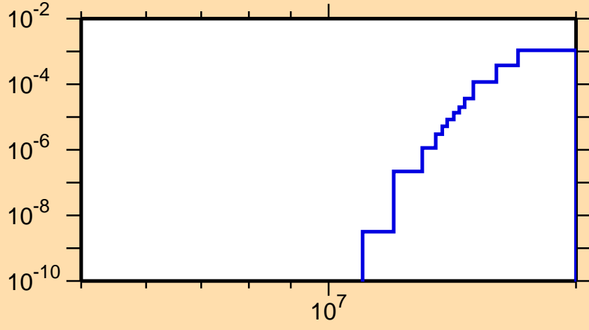
\sigma vs. E for ^{177}\text{Tm}(n,np)
