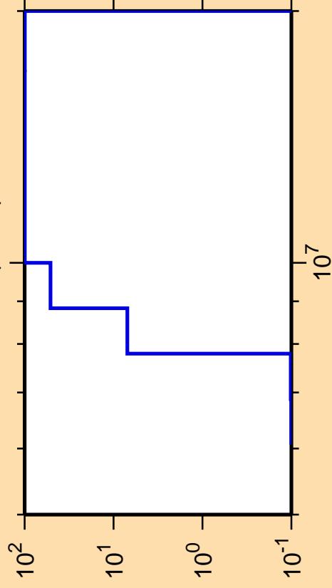
\Delta\sigma/\sigma vs. E for ^{177}\text{Tm}(n,n\alpha)
