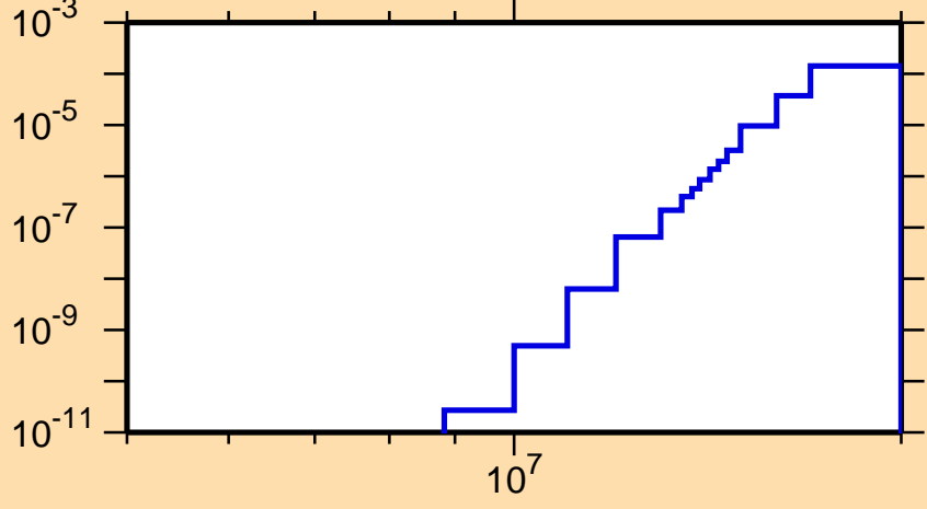
\sigma vs. E for ^{177}\text{Tm}(n,n\alpha)
