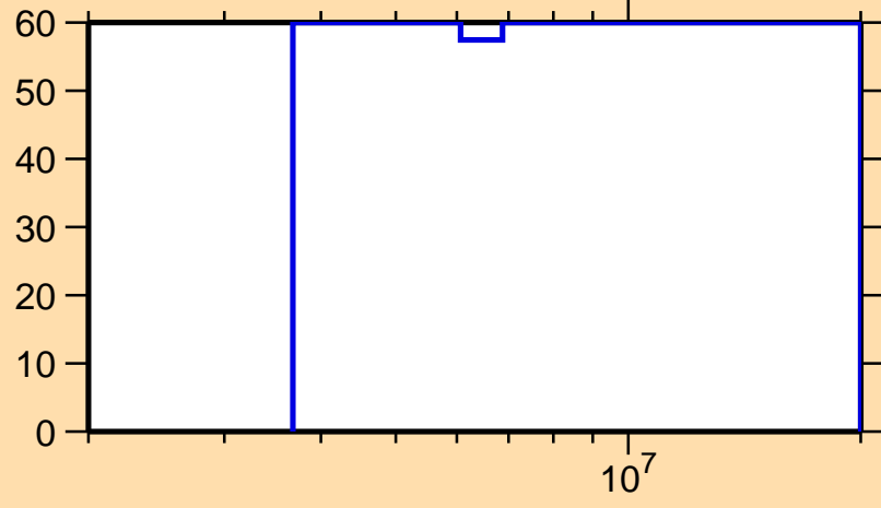
\Delta\sigma/\sigma vs. E for ^{177}\text{Tm}(n,\gamma)
