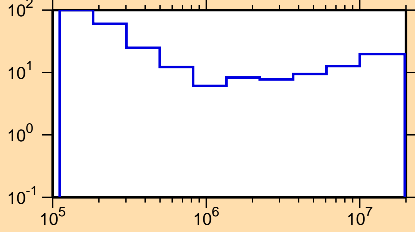
\Delta\sigma/\sigma vs. E for ^{177}\text{Tm}(n,\text{nonel.})
