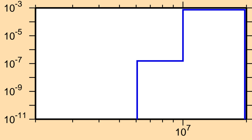
\sigma vs. E for ^{177}\text{Tm}(n,p)
