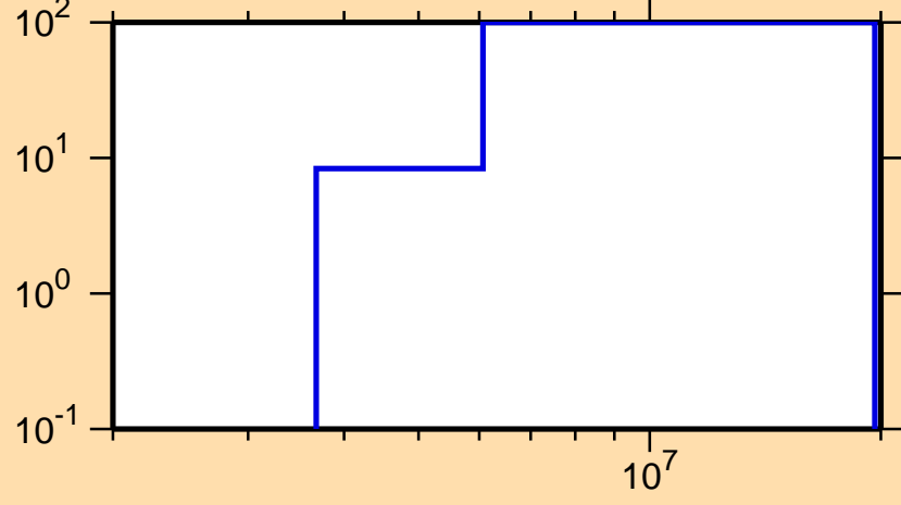
\Delta\sigma/\sigma vs. E for ^{177}\text{Tm}(n,ncont.)
