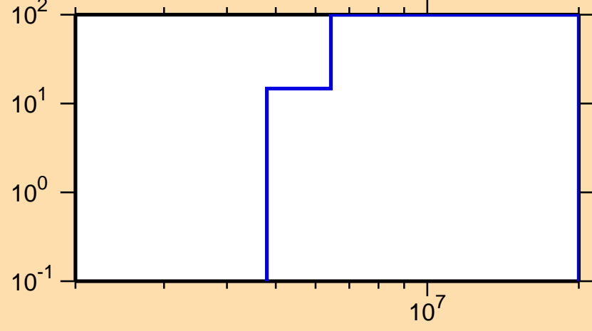
\Delta\sigma/\sigma vs. E for ^{177}\text{Tm}(n,\text{inel.})
