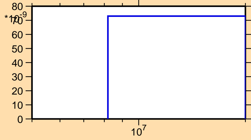
\sigma vs. E for ^{177}\text{Tm}(n,nt)
