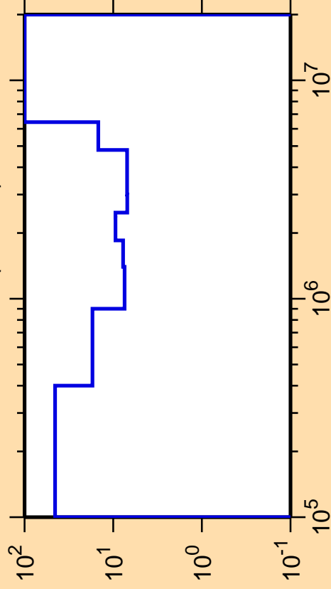
\Delta\sigma/\sigma vs. E for ^{177}\text{Tm}(n,\text{inel.})
