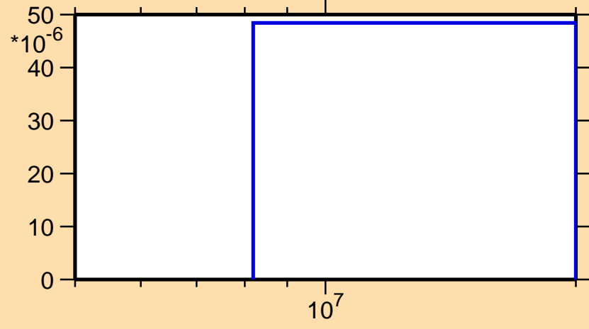
\sigma vs. E for ^{177}\text{Tm}(n,d)
