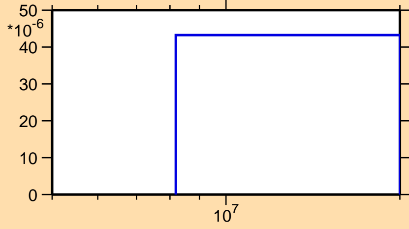
\sigma vs. E for ^{177}\text{Tm}(n,np)
