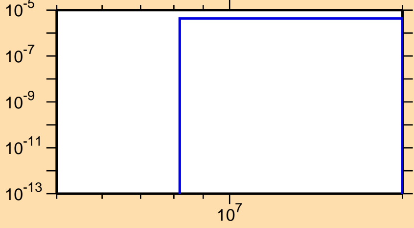
\sigma vs. E for ^{177}\text{Tm}(n,\alpha)
