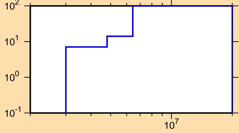
\Delta\sigma/\sigma vs. E for ^{177}\text{Tm}(n,ncont.)
