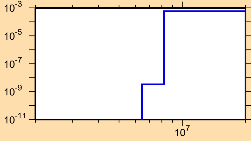
\sigma vs. E for ^{177}\text{Tm}(n,p)
