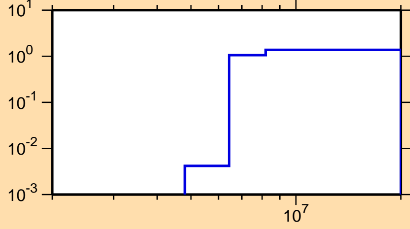
\sigma vs. E for ^{177}\text{Tm}(n,2n)
