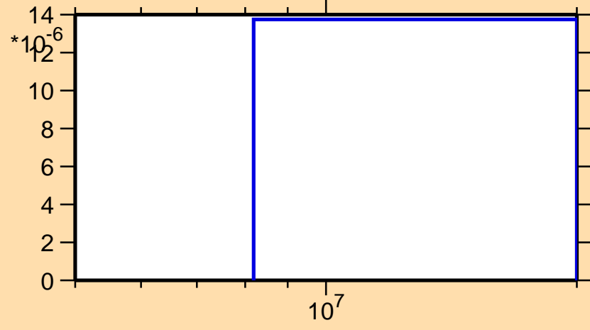
\sigma vs. E for ^{177}\text{Tm}(n,t)
