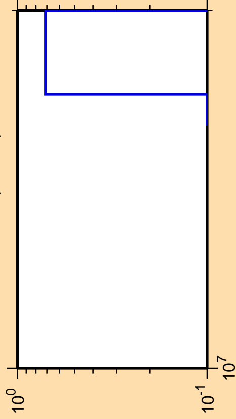
\Delta\sigma/\sigma vs. E for ^{178}\text{Tm} (mt 11)
