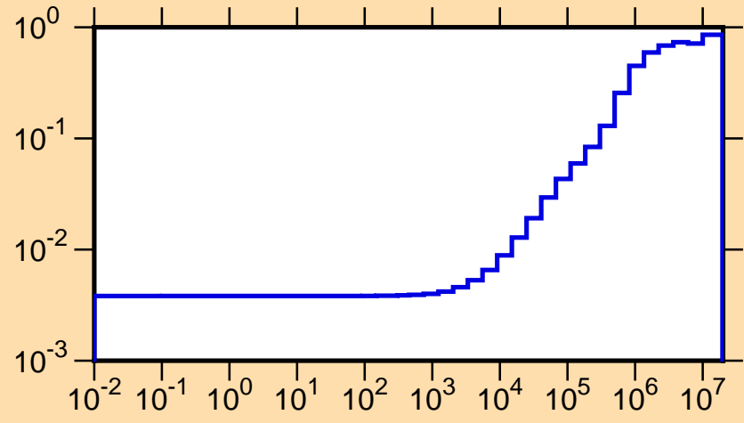
\mu vs. E for ^{178}\text{Tm}(\text{mt251})
