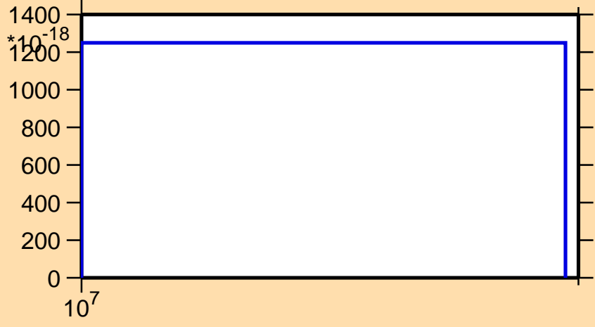
\sigma vs. E for ^{178}\text{Tm}(n,3n\alpha)
