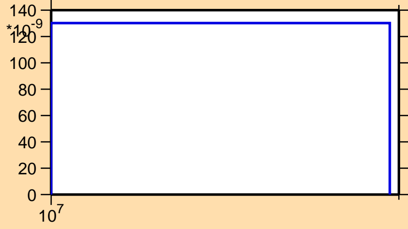
\sigma vs. E for ^{178}\text{Tm}(n,nd)
