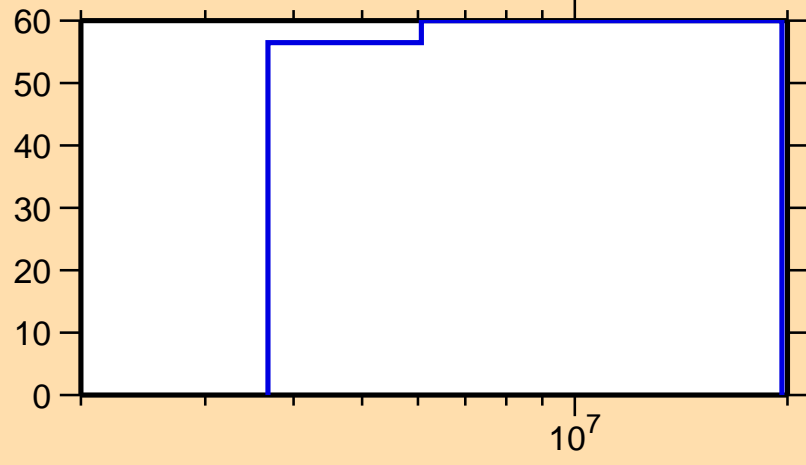
\Delta\sigma/\sigma vs. E for ^{178}\text{Tm}(n,\text{inel.})
