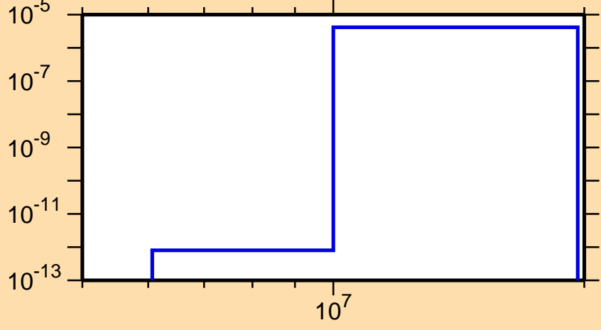
\sigma vs. E for ^{178}\text{Tm}(n,n\alpha)
