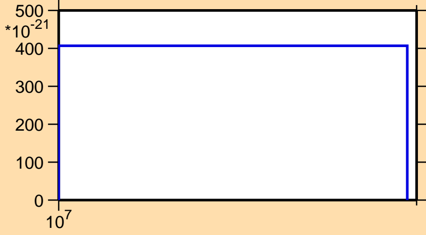
\sigma vs. E for ^{178}\text{Tm} (mt 42)
