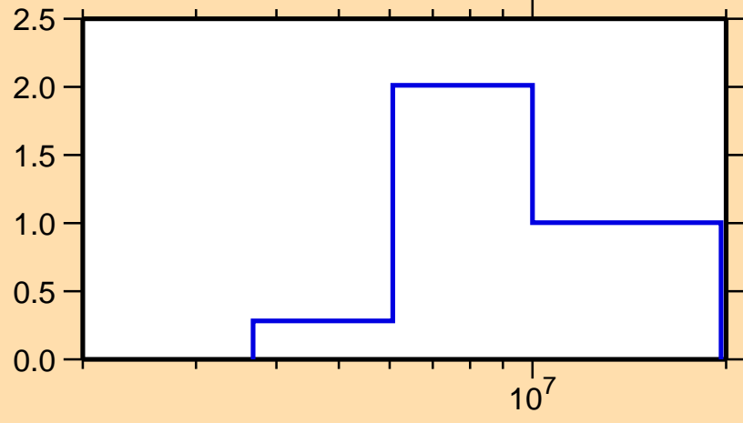
\sigma vs. E for ^{178}\text{Tm}(n,2n)
