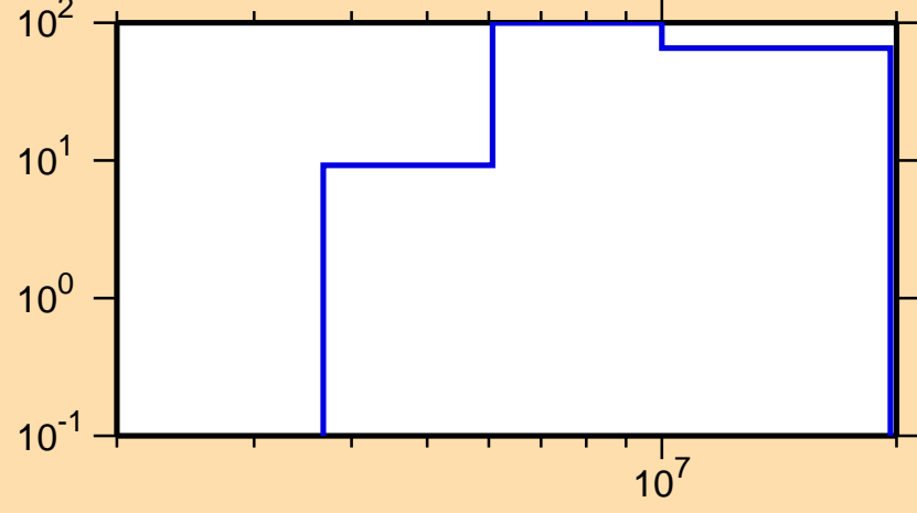
\Delta\sigma/\sigma vs. E for ^{178}\text{Tm}(n,p)
