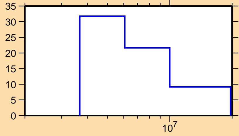
\Delta\sigma/\sigma vs. E for ^{178}\text{Tm}(n,\text{el.})
