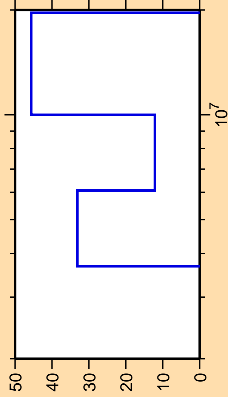
\Delta\sigma/\sigma vs. E for ^{178}\text{Tm}(n,2n)
