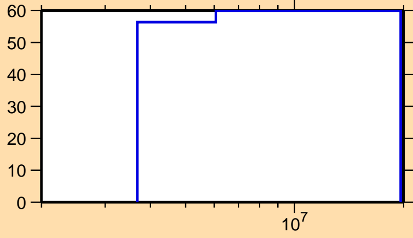
\Delta\sigma/\sigma vs. E for ^{178}\text{Tm}(n,ncont.)
