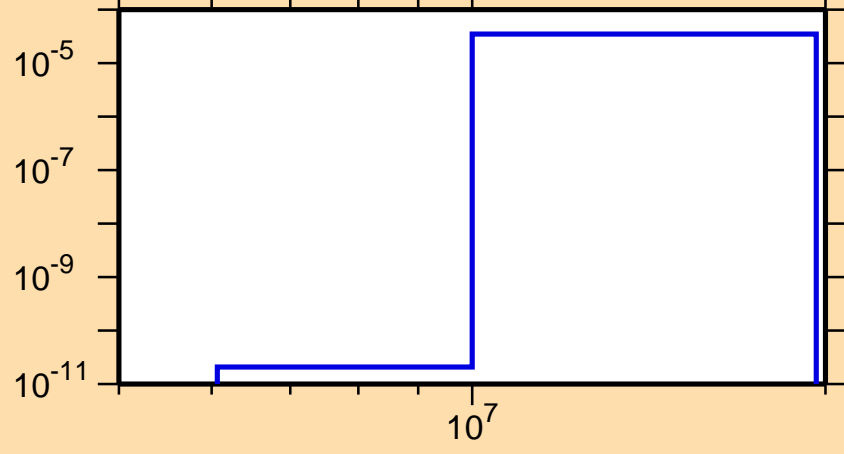
\sigma vs. E for ^{178}\text{Tm}(n,t)
