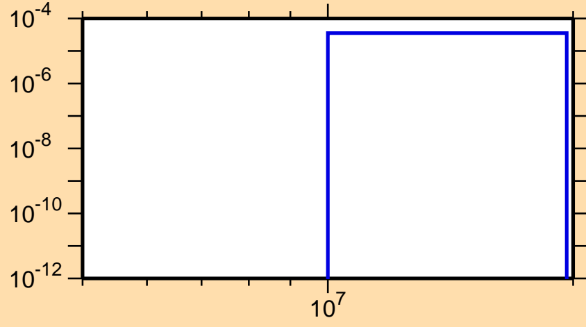
\sigma vs. E for ^{178}\text{Tm}(n,np)
