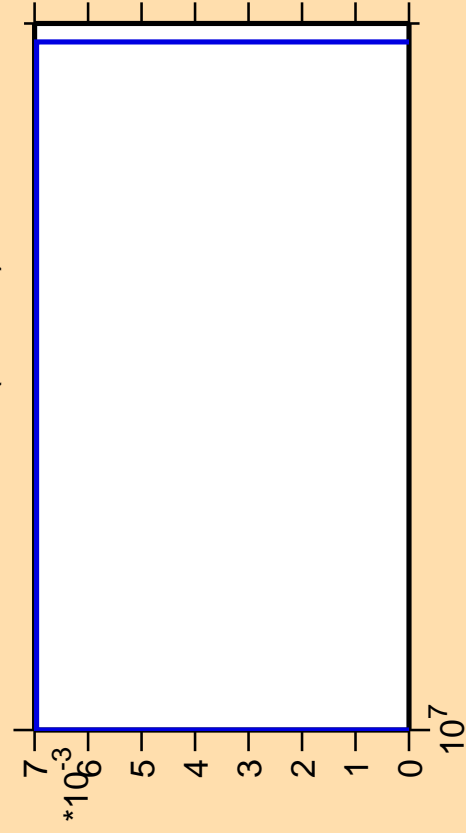
\Delta\sigma/\sigma vs. E for ^{178}\text{Tm}(n,3n\alpha)
