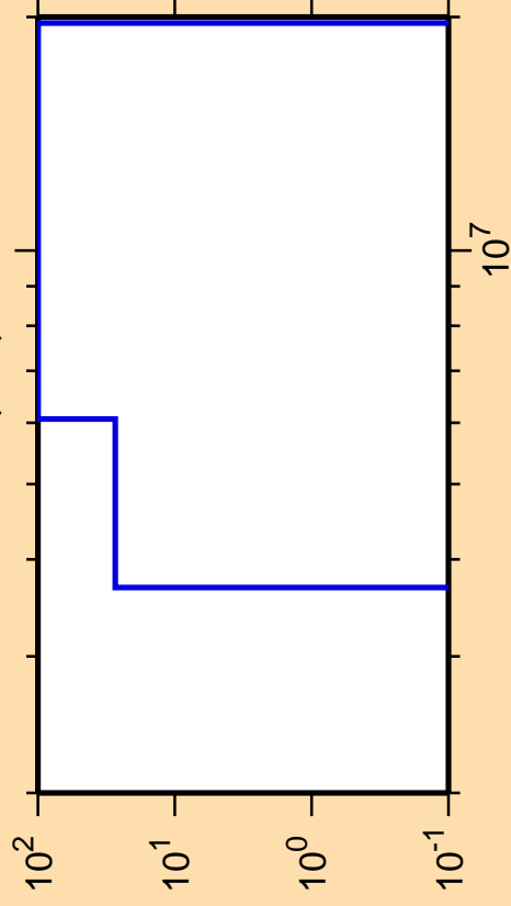
\Delta\sigma/\sigma vs. E for ^{178}\text{Tm}(n,\alpha)
