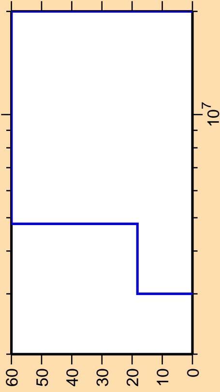
\Delta\sigma/\sigma vs. E for ^{178}\text{Tm}(n,n\text{cont.})
