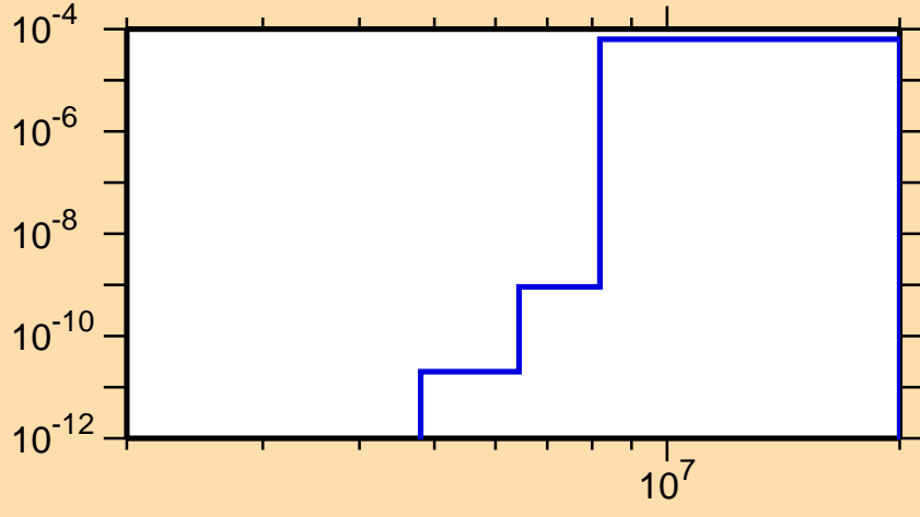
\sigma vs. E for ^{178}\text{Tm}(n,\alpha)
