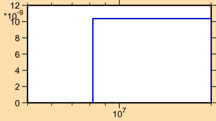
\sigma vs. E for ^{178}\text{Tm}(n,2np)
