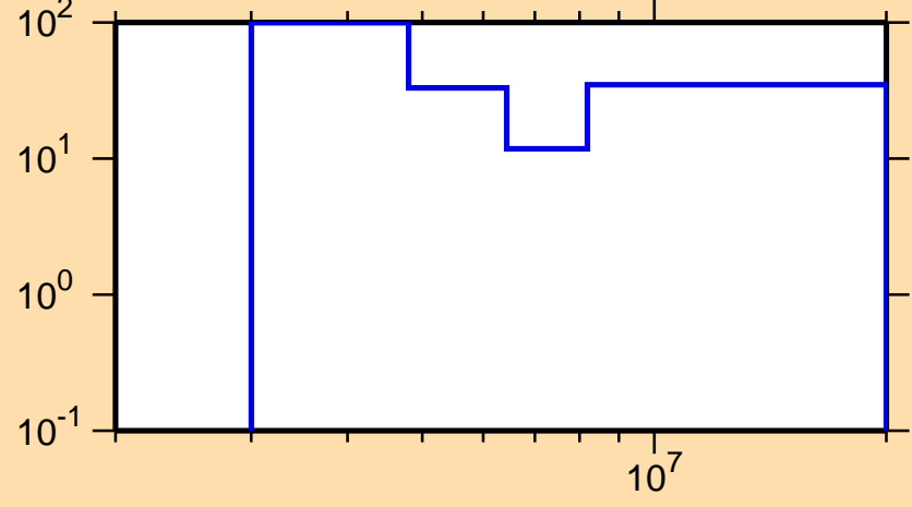
\Delta\sigma/\sigma vs. E for ^{178}\text{Tm}(n,2n)
