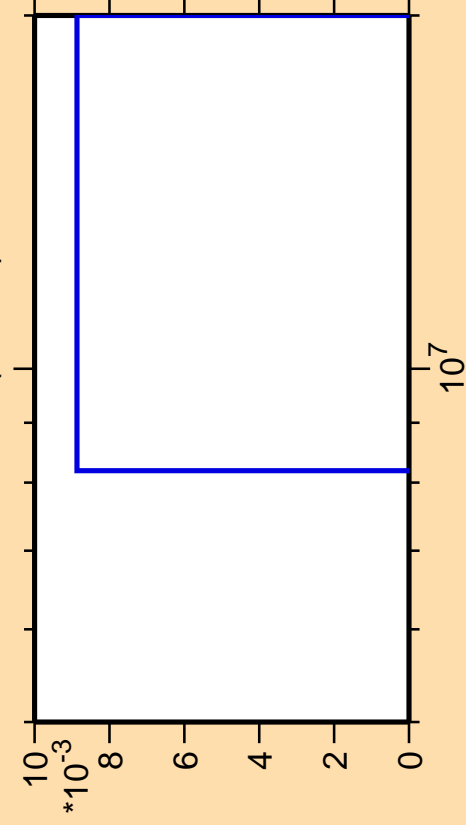
\Delta\sigma/\sigma vs. E for ^{178}\text{Tm}(n,3n\alpha)
