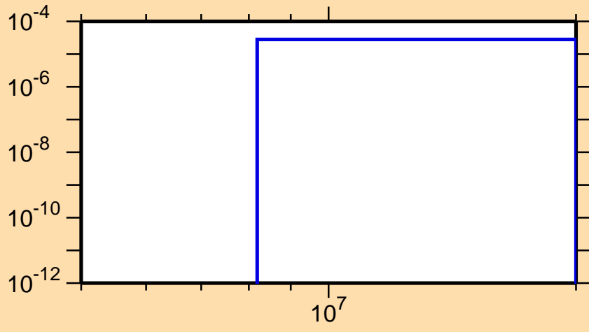
\sigma vs. E for ^{178}\text{Tm}(n,t)
